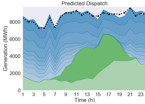
Fig. 4: Stacked plot of a single day’s predicted dispatch for all conventional generators (blue) and for all renewable generators (green). The aggregated load is indicated by the black dotted line.
