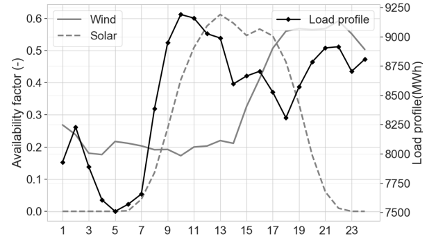
Fig. 3: The availability factor of the renewable energy sources, i.e., the wind and solar generation (left-axis), and the aggregated demand in the system (right-axis) throughout an example day.
