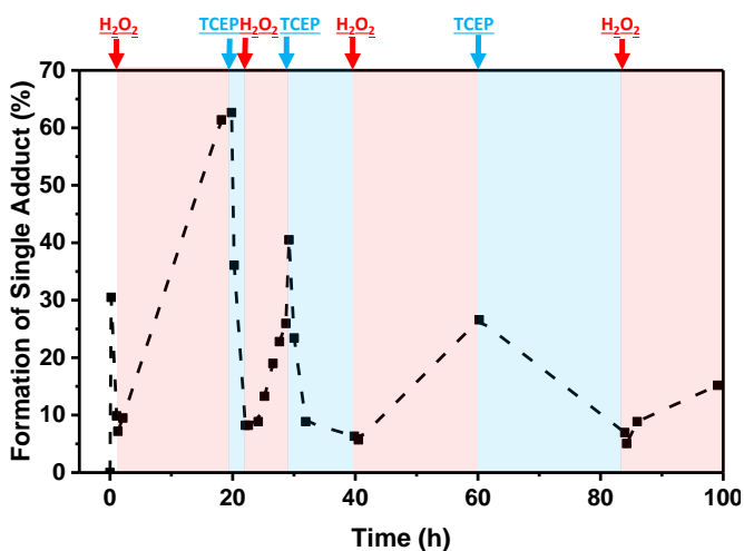
Figure S4.4. ^1\text{H-NMR} (399.7 MHz, 298 K in \text{D}_2\text{O} / PB8.2=1:9) monitoring of the redox-responsive thiol-alkynone double addition between 3-butyln-2-one 1 and BME 2 in PB8.2 reversibly controlled by \text{H}_2\text{O}_2 and TCEP. Spectrum 1 shows that the double adduct was generated after mixing 3-butyln-2-one 1 and BME 2 . Spectrum 2, 4, 6 show after the first, second, third and fourth time of addition of \text{H}_2\text{O}_2 , the double adduct 4 was converted to the single adduct 3 . Spectrum 3, 5, 7 show after the first, second and third time of addition of TCEP, the single adduct 3 was converted to the double adduct 4 .
