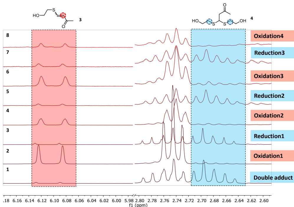
Figure S4.4. ^1\text{H-NMR} (399.7 MHz, 298 K in \text{D}_2\text{O} / PB8.2=1:9) monitoring of the redox-responsive thiol-alkynone double addition between 3-butyln-2-one 1 and BME 2 in PB8.2 reversibly controlled by \text{H}_2\text{O}_2 and TCEP. Spectrum 1 shows that the double adduct was generated after mixing 3-butyln-2-one 1 and BME 2 . Spectrum 2, 4, 6 show after the first, second, third and fourth time of addition of \text{H}_2\text{O}_2 , the double adduct 4 was converted to the single adduct 3 . Spectrum 3, 5, 7 show after the first, second and third time of addition of TCEP, the single adduct 3 was converted to the double adduct 4 .
