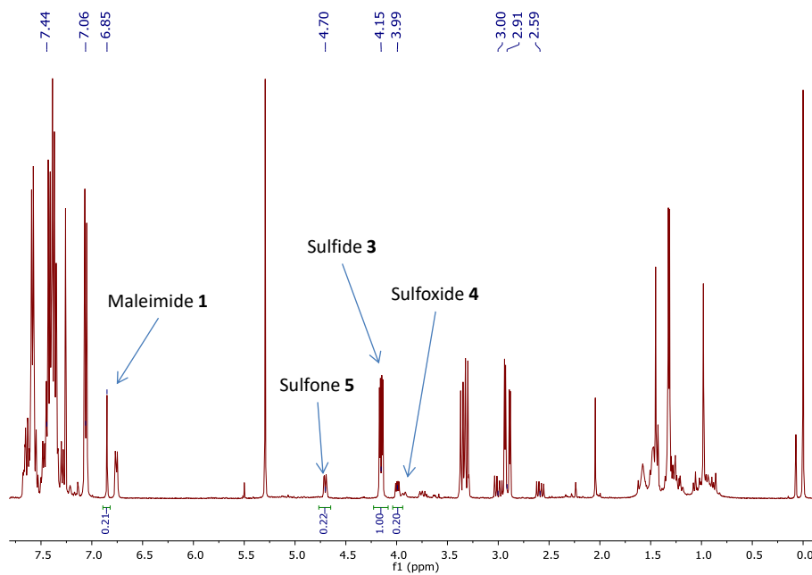
Figure S2.10. ^1\text{H} NMR (399.7 MHz, 298 K in \text{CDCl}_3 ) spectrum of product mixture after oxidation by \text{H}_2\text{O}_2 with vanadium complex catalyst.
