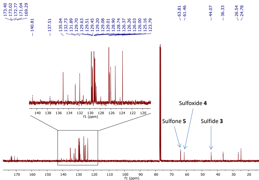
S2.4. ^{13}\text{C} NMR (100.5 MHz, 298 K in \text{CDCl}_3 ) spectrum of the oxidation product \text{S}_1 .
