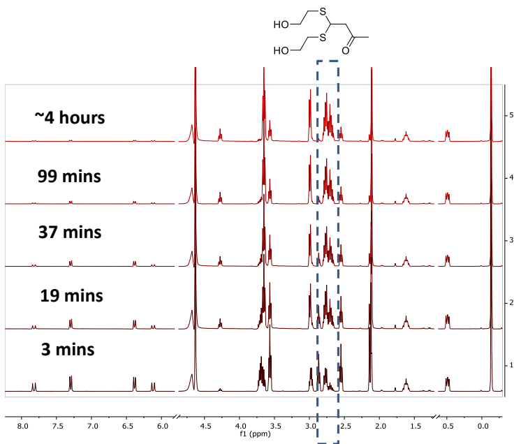
Figure S3.10. 1 H-NMR (399.7 MHz, 298 K in D 2 O/PBS, 4 drops of D 2 O in 1 mL PBS7.4) monitoring of thiol-alkynone double reaction between 3-buten-2-one and 2-mercaptoethanol in PBS7.4.
