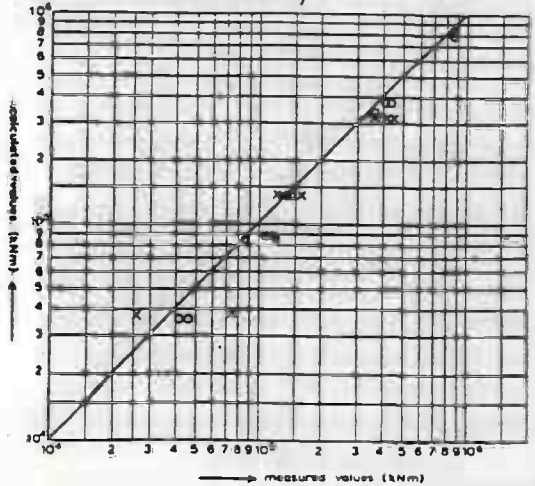
CALCULATED AND EXPERIMENTAL DATA FOR M_z
