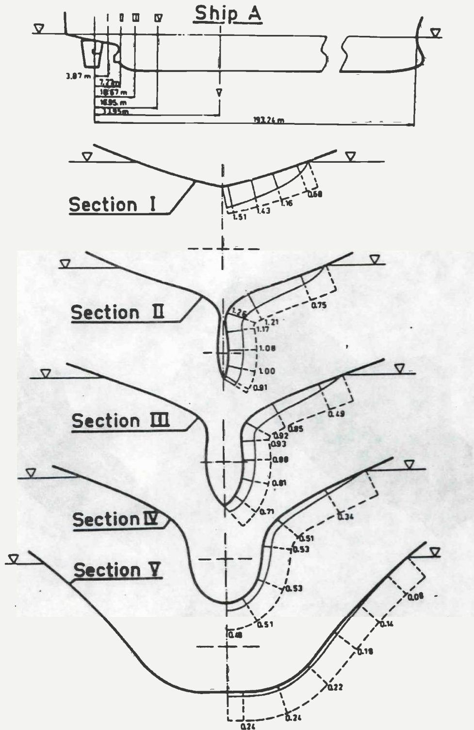
FIGURE 9 - EXAMPLE OF VARIATION OF SOLID BOUNDARY FACTORS, INCLUDING INFLUENCE FROM FREE SURFACE EFFECTS, REF. 59. DOTTED LINES REPRESENT THE VALUE S = 2.0
