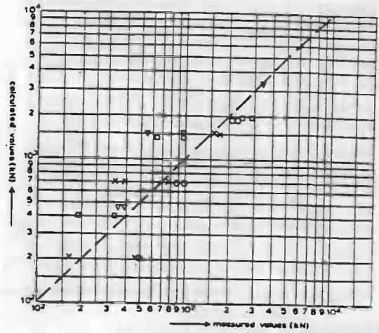
CALCULATED AND EXPERIMENTAL DATA FOR F_x
