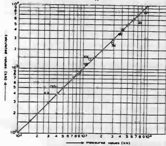
CALCULATED AND EXPERIMENTAL DATA OF F_y
