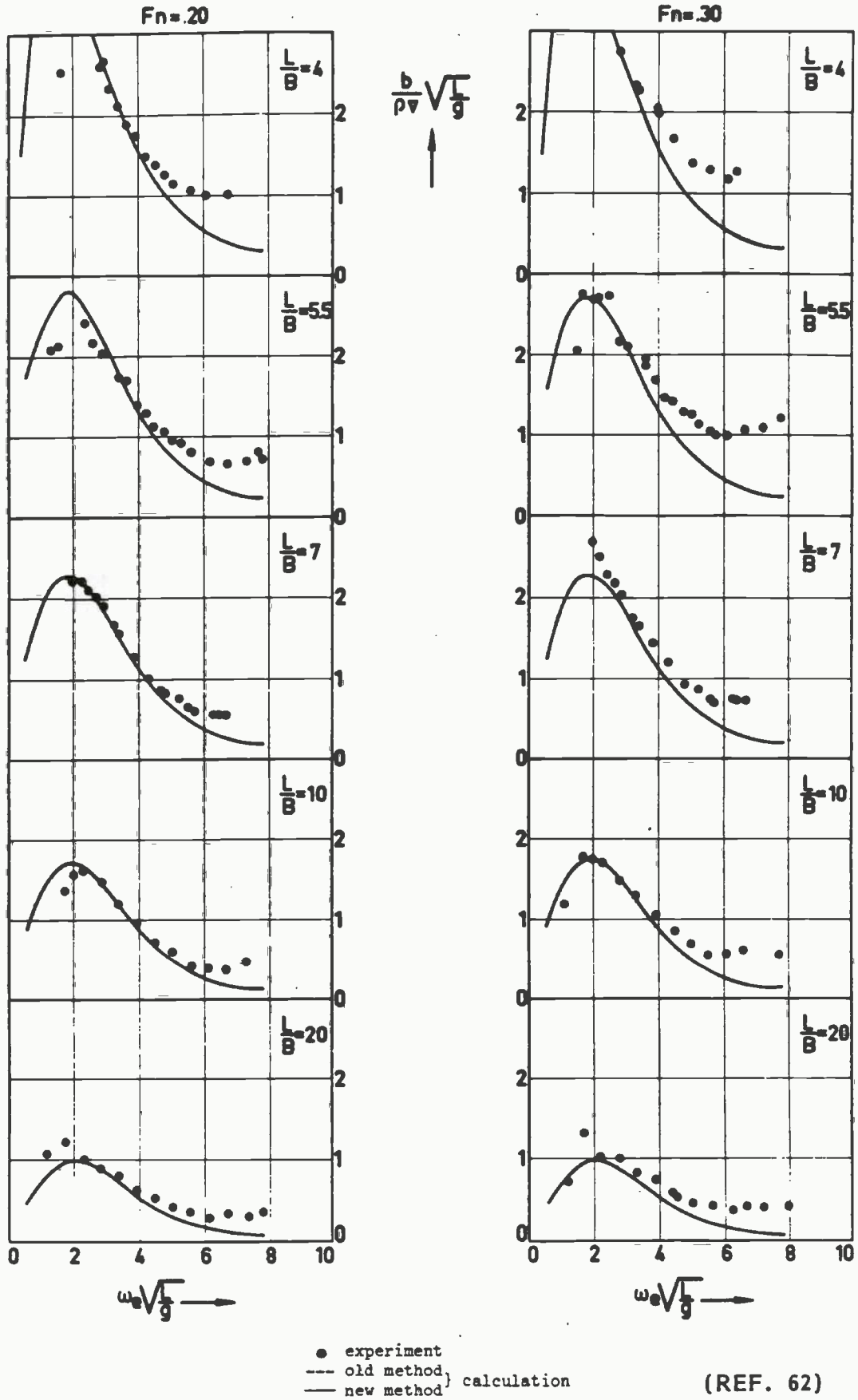
FIGURE 12 - HEAVE DAMPING COEFFICIENT
