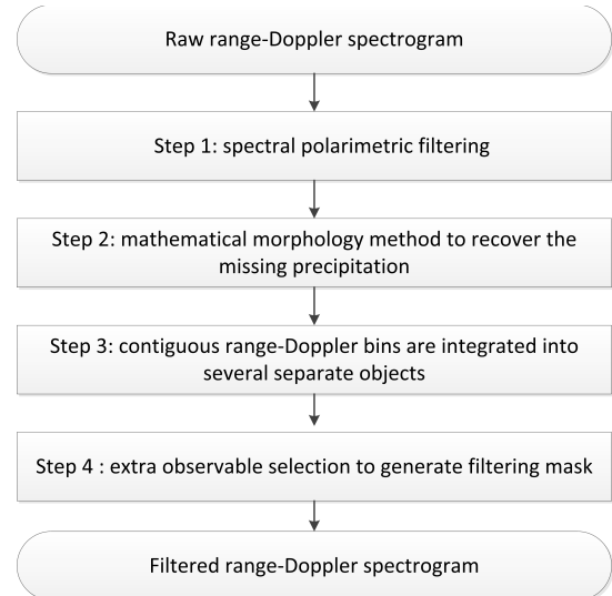
Fig. 6. Flowchart of the OBSpol filter applied to RFI mitigation.
