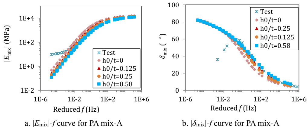
Fig. 12. The sensitivity of predicted |E_{mix}| and \delta_{mix} on h_0 .
