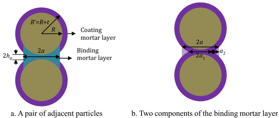
Fig. 6. Illustration of binding mortar layers.
