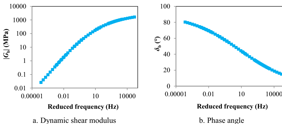
Fig. 10. Measured shear modulus of mortar.
