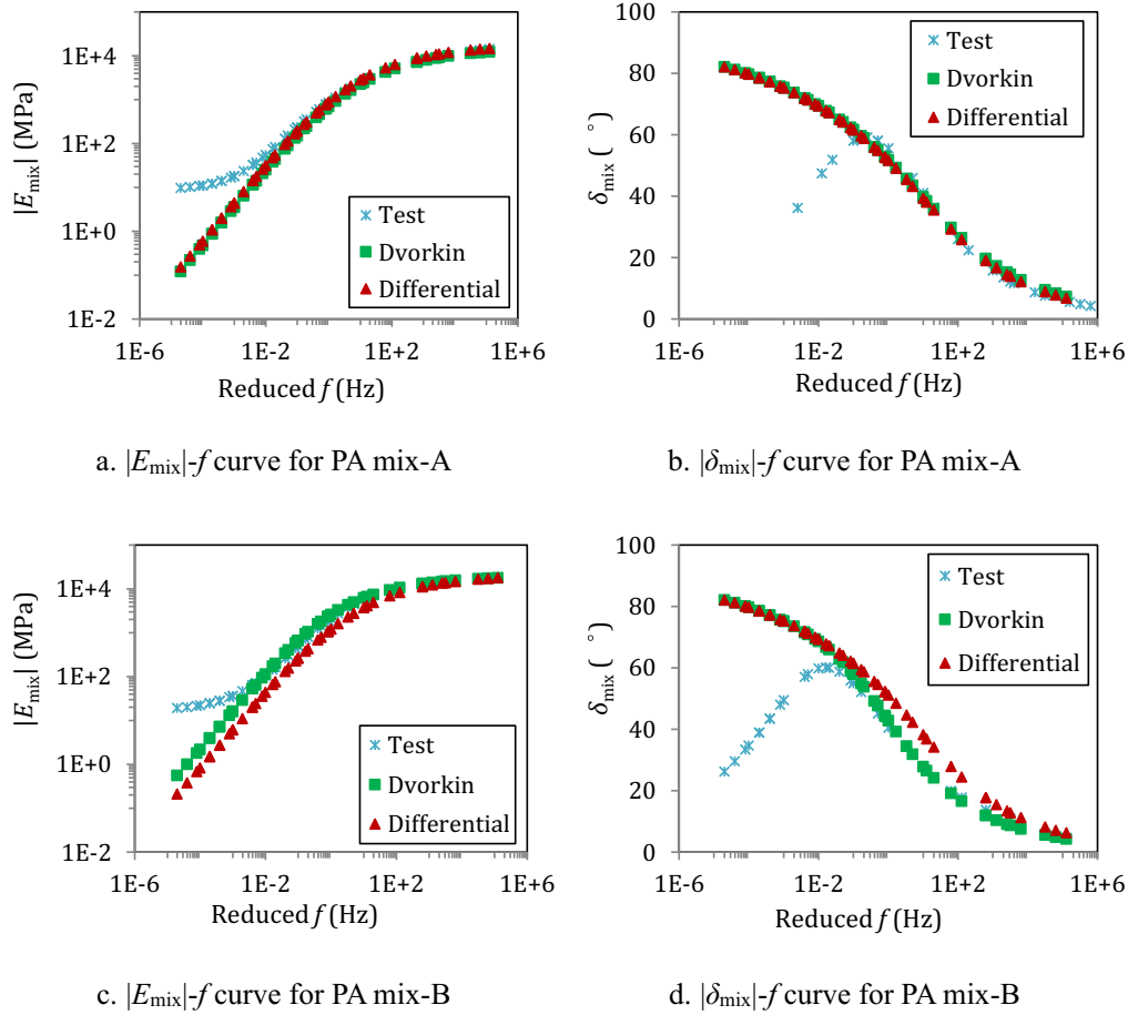
Fig. 11. Comparison of tested and predicted E_{mix} .
