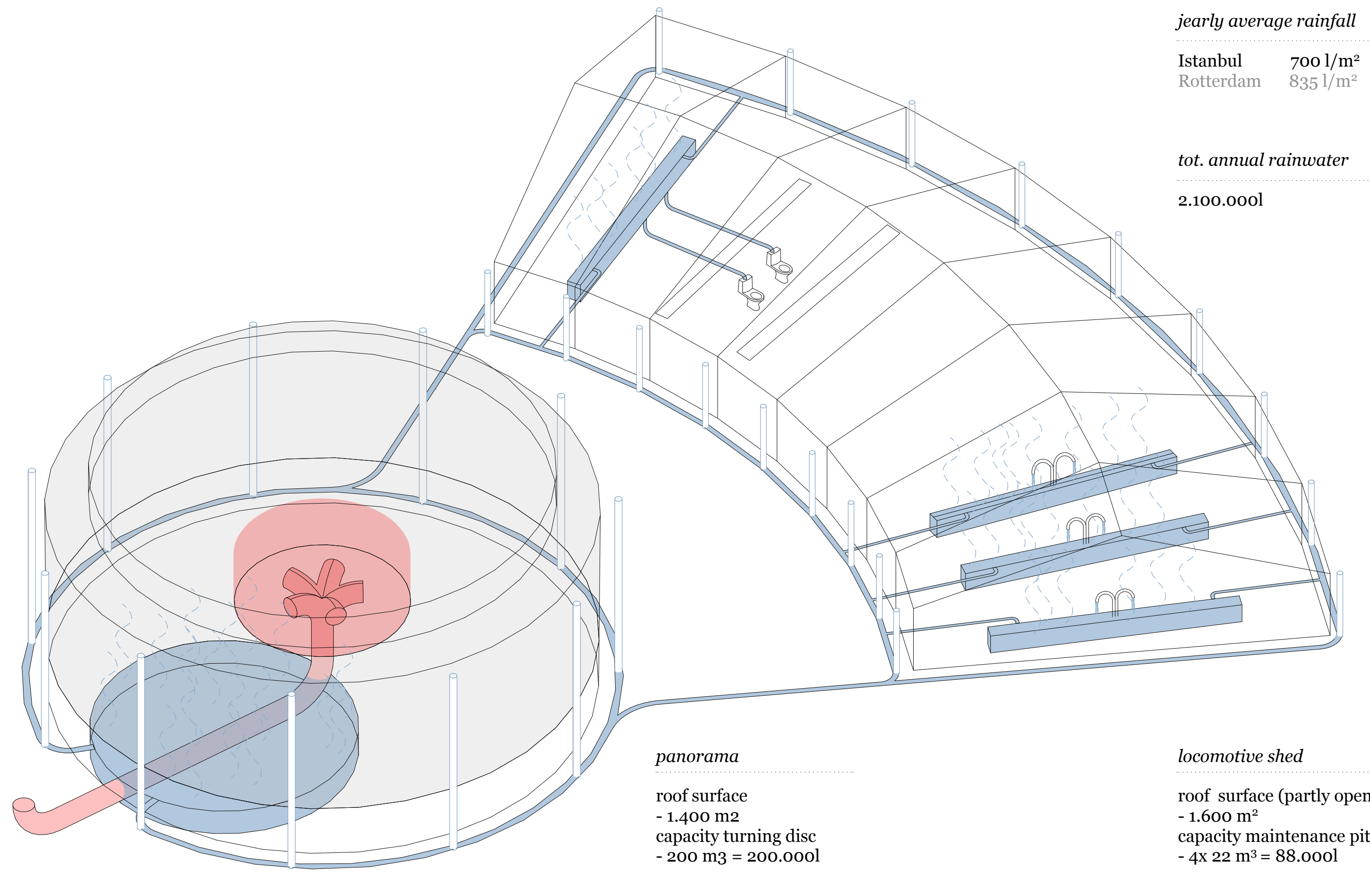
water and climate diagram
