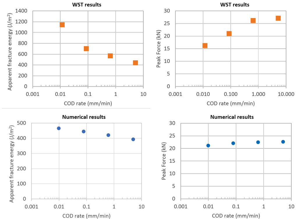
Figure 8: Peak horizontal force ( F_H ) and apparent fracture energy ( G_f^I ) as a function of the COD rate. Top, experimental results. Bottom, numerical modelling results.
