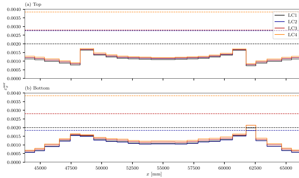
Fig. 17. Imposed ASR expansion in longitudinal direction x ( \epsilon_x^{\text{asr}} ) in the outer beam of span 3 for all load combinations. Dashed lines are the corresponding free ASR expansion ( \epsilon_x^{\text{asr,free}} ).
