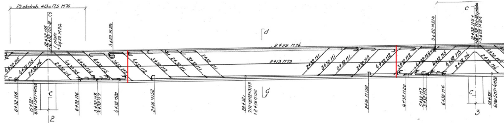
Fig. 9. Drawing of the reinforcement in the mid span beams of Elegeseter bridge [39]. The cross sections with low amount of reinforcement are marked in red. (For interpretation of the references to colour in this figure legend, the reader is referred to the web version of this article.)
