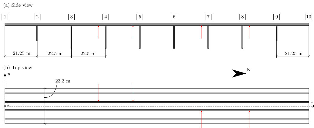
Fig. 6. Drawing of Elgeseter bridge. The locations of large cracks (crack widths up to 6 mm) are marked with red arrows. Source: Adapted from [38].
