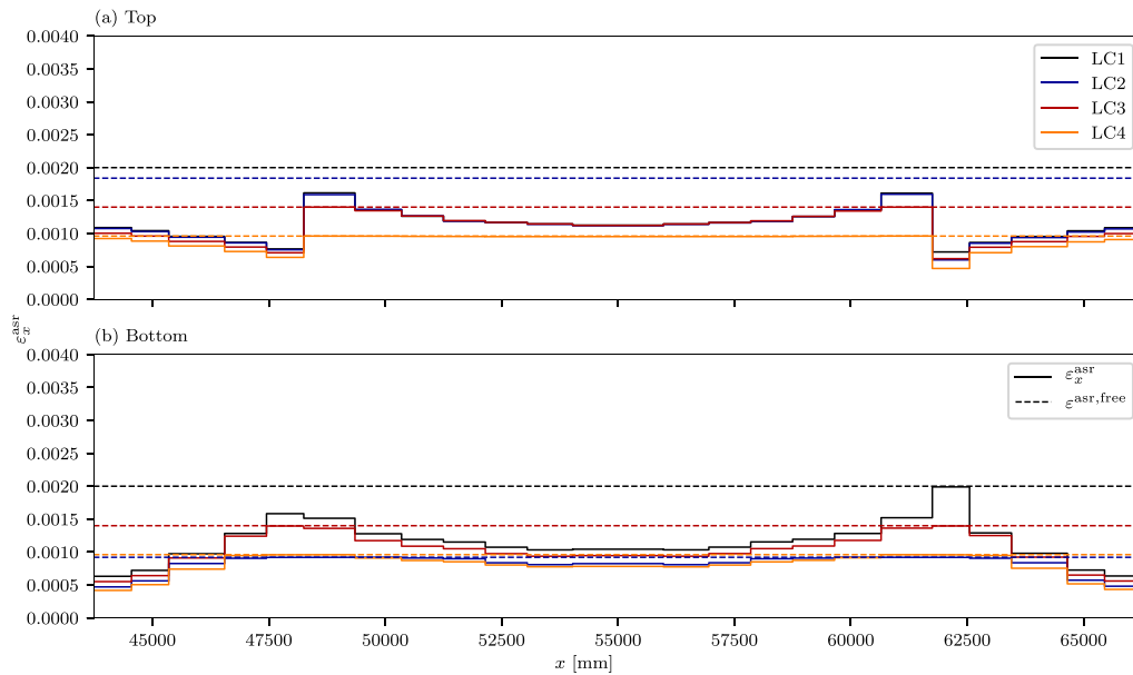
Fig. 18. Imposed ASR expansion in longitudinal direction x ( \epsilon_x^{\text{asr}} ) in the inner beam of span 3 for all load combinations. Dashed lines are the corresponding free ASR expansion ( \epsilon_x^{\text{asr,free}} ).
