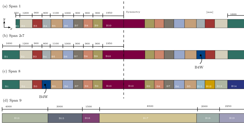
Fig. 12. The beams are divided into regions and assigned different shell sections with different reinforcement amounts. In span 2-8, one week section, B4W, is included with only three \phi 32 bars in the bottom of the beam (approx 4.5 m from the columns, as observed on the bridge).
