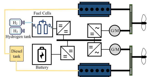
(b) Initial proposed hybrid propulsion powertrain
