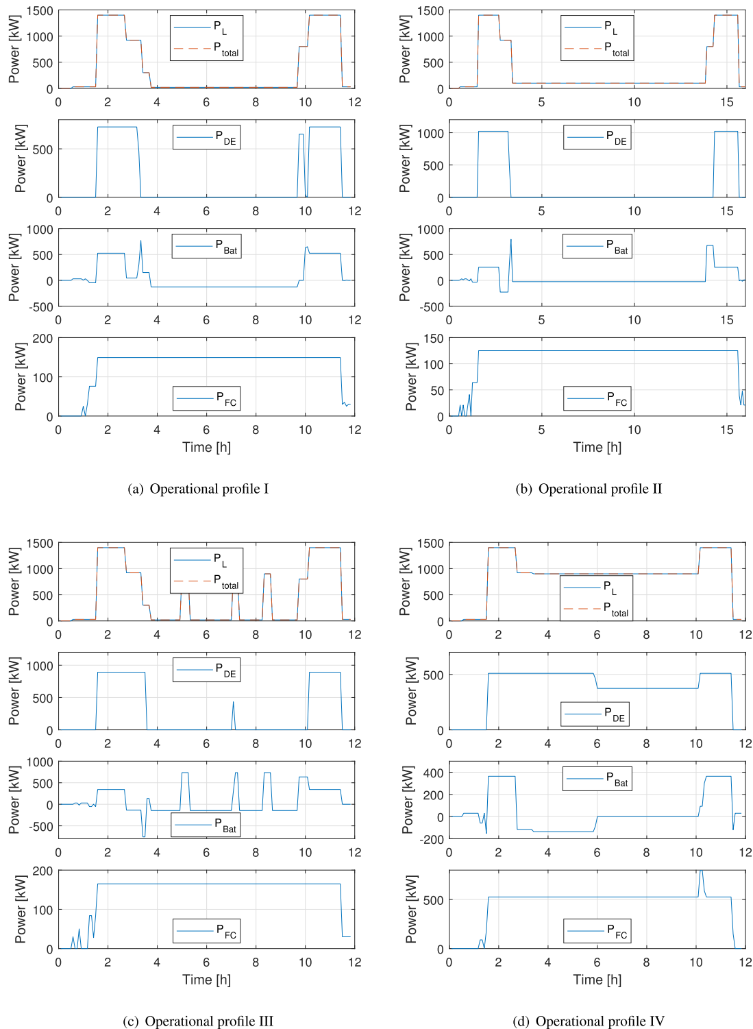
FIGURE 21. Power schedule of the selected designs for medium emission reduction.
