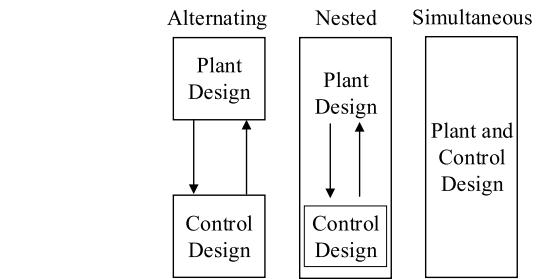
FIGURE 2. System level optimization architectures [20].
