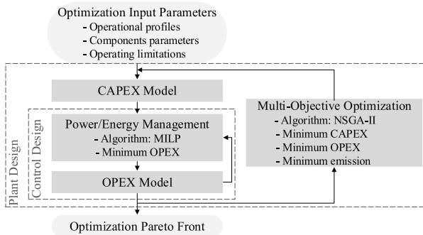
FIGURE 9. Optimization procedure.
