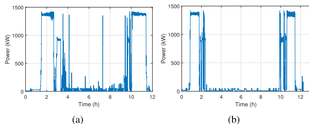
FIGURE 6. Operational profile measured on-site.
