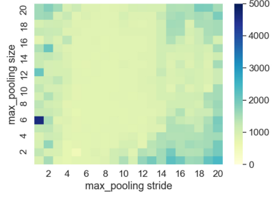
(b) T_{GE0} : tuning the first max-pooling layer (min: 527; max: 4 616)
