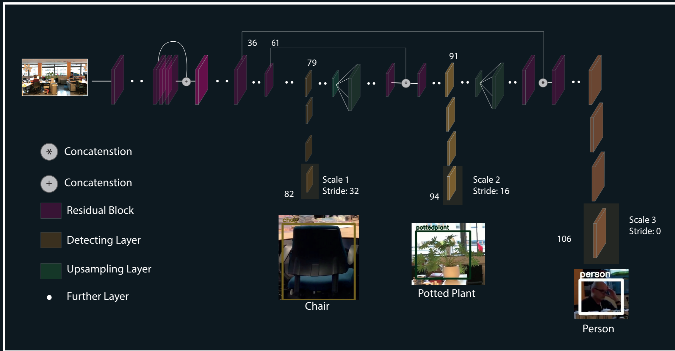
Yolo- V3 Network Architechture
