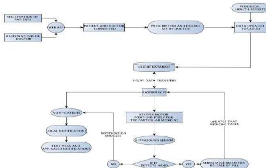
Figure 2: Control Flow Diagram
