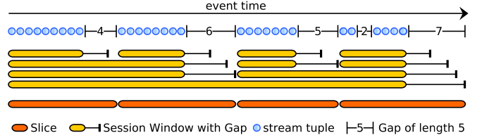
Fig. 2: Session Window Aggregate Sharing.
