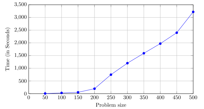
Fig. 6. CPU time taken to obtain optimal solutions (in seconds).
