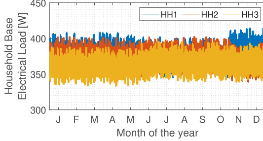
Fig. 5. The three household load profiles used in this study based on publicly available data on the electricity demand of Dutch private dwellings [24].
