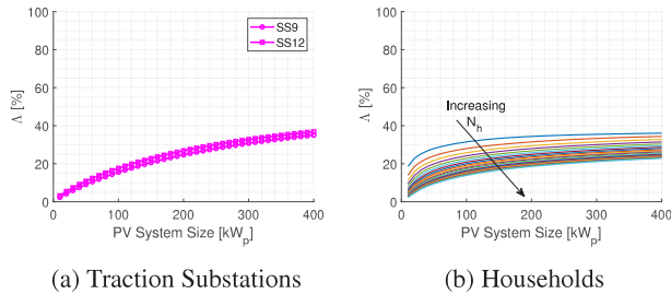
Fig. 11. Direct Load Coverage by a PV system connecting only to a traction substation or to households.
