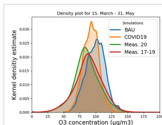
Figure 3. PDFs of ozone concentration at all 'rural'/rural-remote' background stations for the BAU and COVID19 simulations as well as for the measurements of 2020 and the combinations of all measurements 2017–2019 (for the period 15 March–31 May).
