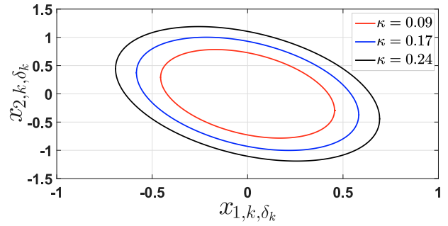
Figure 4. Ellipsoid \mathcal{E}_x for different values of \kappa .
