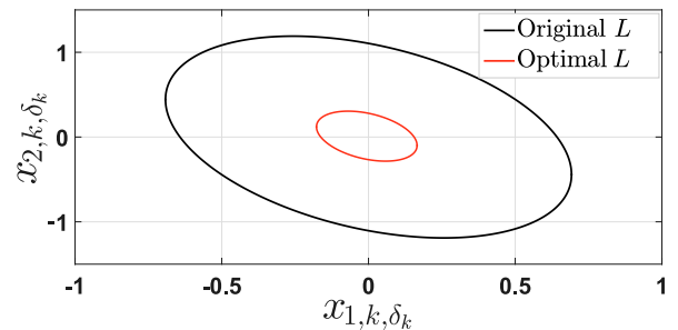
Figure 6. The improvement in the hidden reachable set ellipsoidal bound \mathcal{E}_x through application of Corollary 2 to design the optimal observer gain.
