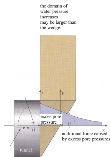
Figure 4 The effect of removal of the cake sealing during excavation on pore-pressures in the front. The influence zone for excess pore-pressures may be larger that the zone normally considered in stability analysis.
