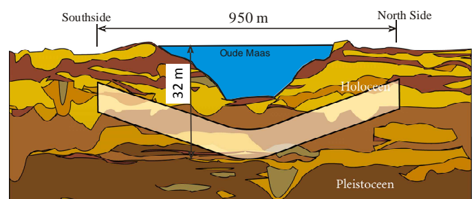
Figure 1. Geological profile at the 2 nd Heinenoord tunnel
