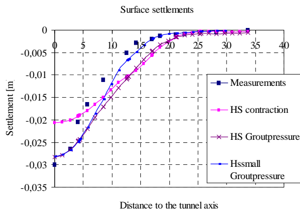
Figure 6. Surface settlements; measured and back-calculated with different material models
