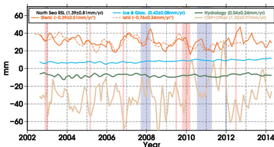
Fig. 19. Estimated sea-level contributions in the North Sea from a combination of GRACE and Jason-1/2 altimeter data. The variability in the North Sea is mostly dominated by ocean bottom pressure changes, which induce the largest uncertainties in the estimated trends (from Rietbroek et al., 2016, supplement).
