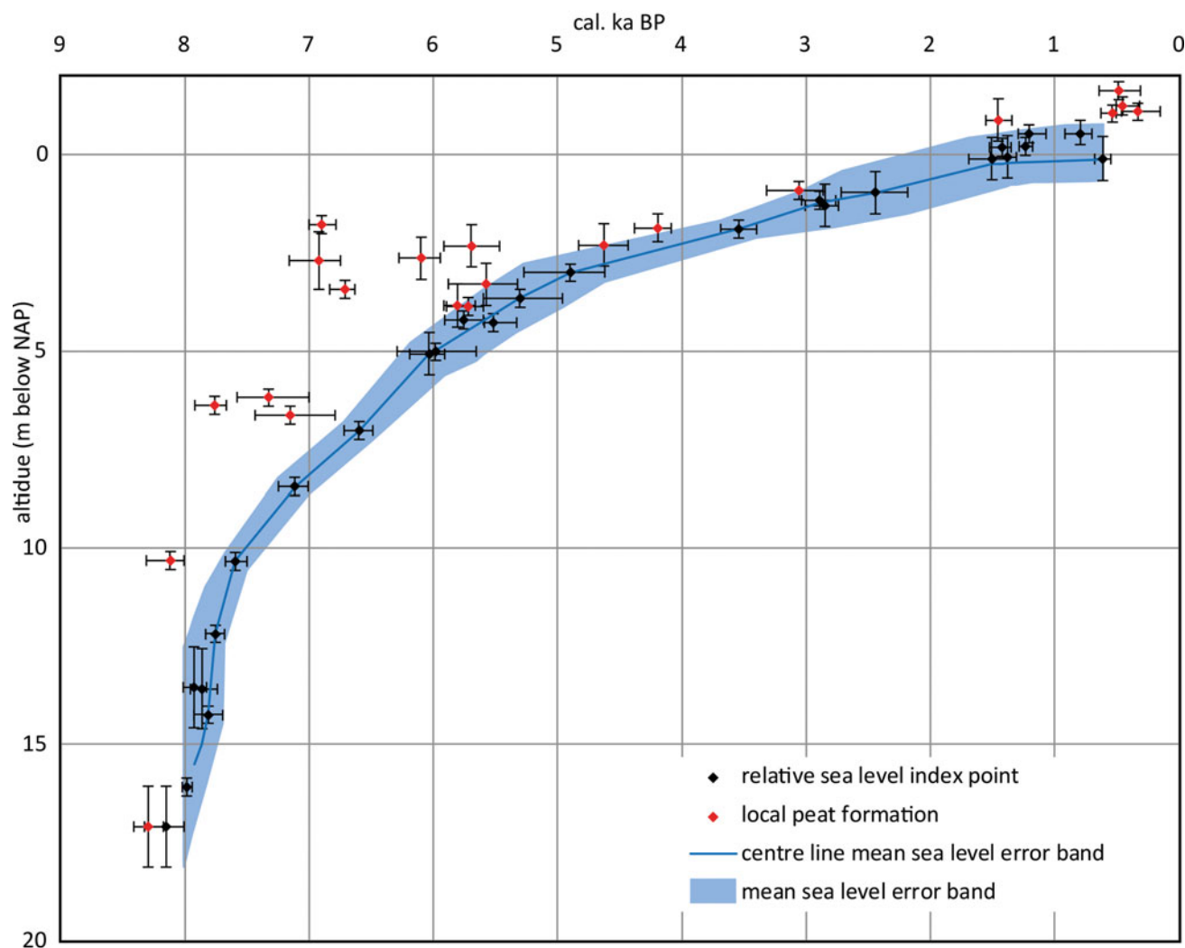
Fig. 11. Time–depth diagram of the 51 originally selected radiocarbon-dated basal peat samples in the Northern Netherlands coastal area. The age ('cal. ka BP') is in years before present, the altitude in metres below NAP (Normaal Amsterdams Peil or Dutch Ordnance Level), which is within 0.1 m of present-day MSL. Red dots indicate samples from peat beds that were formed above contemporary sea level and thus cannot be used as sea-level indicators. The 26 index points in the lowest time–depth position (black dots) are interpreted to track sea level and are used for the reconstruction of the sea-level curve and error band. Vertical error bars contain primarily errors in altitude determination but no estimate of the indicative meaning of the index points. See Meijles et al. (accepted) for further details on data selection, evaluation and error term treatment.
