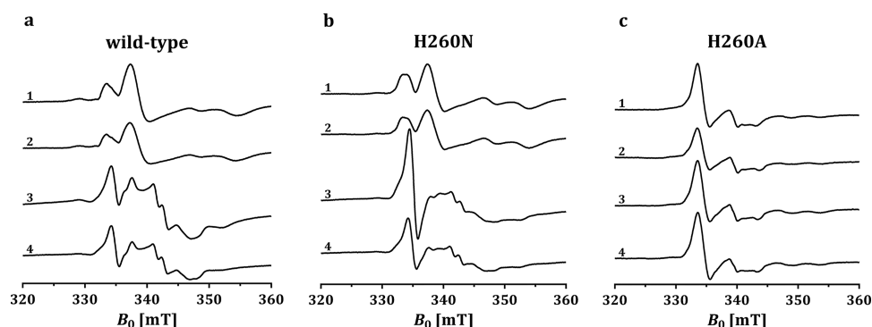
Figure 4. Study of the 77 K EPR signals of wild type Bam(BC) 2 and two variants. (a) Wild type, (b) His260Asn (H260N) variant, and (c) His260Ala (H260A) variant. (1) As isolated, (2) incubated with inhibitor 1-monoenoyl-CoA, (3) incubated with 1,5-dienoyl-CoA at 4 °C for ~1 min, and (4) incubated with 1,5-dienoyl-CoA, for 5 min at room temperature. All spectra were recorded at 5 mW microwave power, 0.3 mT modulation amplitude, 100 kHz modulation frequency, and 81.92 ms conversion time. All spectra were normalized to 9.40 GHz microwave frequency for comparison.
