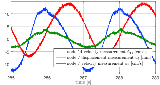
Fig. 3. Simulated displacement at node 7 and velocities at nodes 7 and 14. Introduced noise is 2% of the standard deviation of the respective displacement or velocity.
