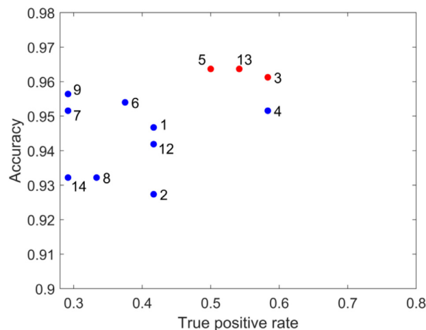
Fig. 7. True positive rates (TPR) and model accuracies (ACC) of 14 trained ML models based on two principal components. Models 3, 5, and 13 are marked in red as they have the best performance for either TPR or ACC. Model numbers correspond to Table 2.
