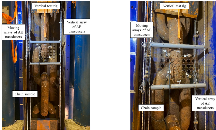
Fig. 3. Instrumented test rig (left) and non-contact sensors deployment in the test rig (right).
