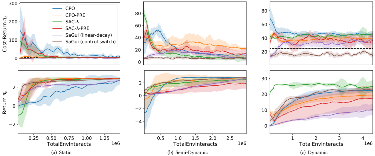
Figure 7: Evaluation of \pi_b for CPO, CPO-PRE, SAC- \lambda , SAC- \lambda -PRE, SaGui (linear-decay), and SaGui (control-switch) over 10 seeds. The black dashed lines indicate the safety thresholds.
