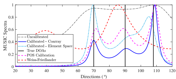
(b) N = 3 , \theta = [70^\circ, 90^\circ, 108^\circ]^T .
