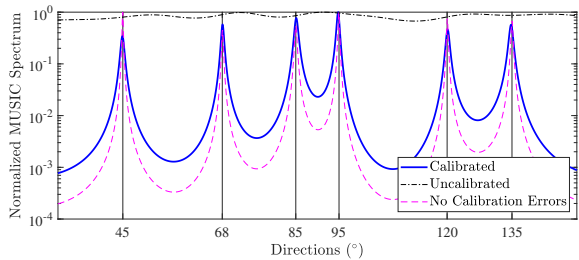
(c) MUSIC spectra with an SNR = 10 dB.
