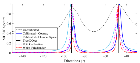
(a) N = 2 , \theta = [-45^\circ, -90^\circ]^T .
