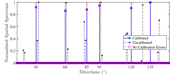
(b) l_1 -SVD spectra with SNR = 10 dB.
