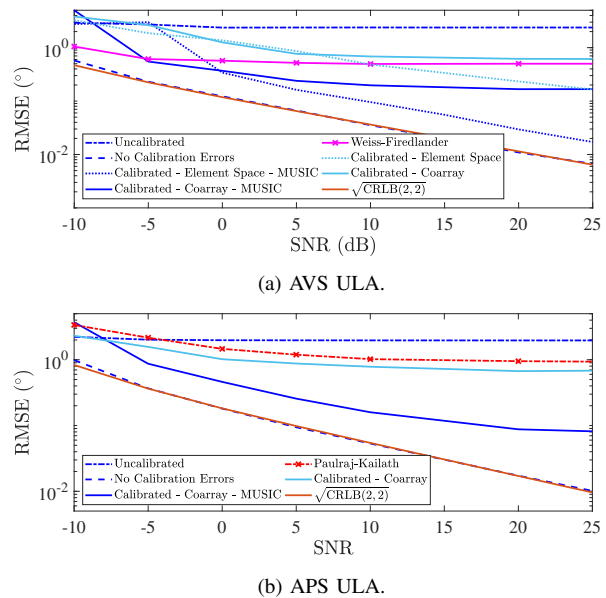
Fig. 7. RMSE variation of the DOA estimates for the source at 90^\circ using both the APS and AVS ULA with M = 8 , N = 3 and \theta = [78^\circ, 90^\circ, 102^\circ] as the SNR varies for a fixed number of snapshots of 1000.
