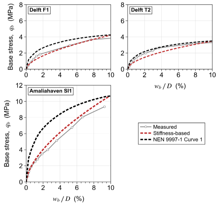
Fig. 8. Prediction of the base mobilisation curves
