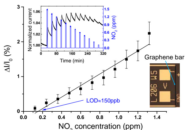
Figure 1: calibration curve of graphene-based chemi-resistive sensor towards NO 2 . Right-down inset shows one device geometry (length=206 \mu\text{m} , width=5 \mu\text{m} ). Current dynamic behavior of sensor upon exposure to 4 min-long gas pulses (left-up inset). The current is normalized to the value I_0 during the gas inlet of the first pulse exposure.
