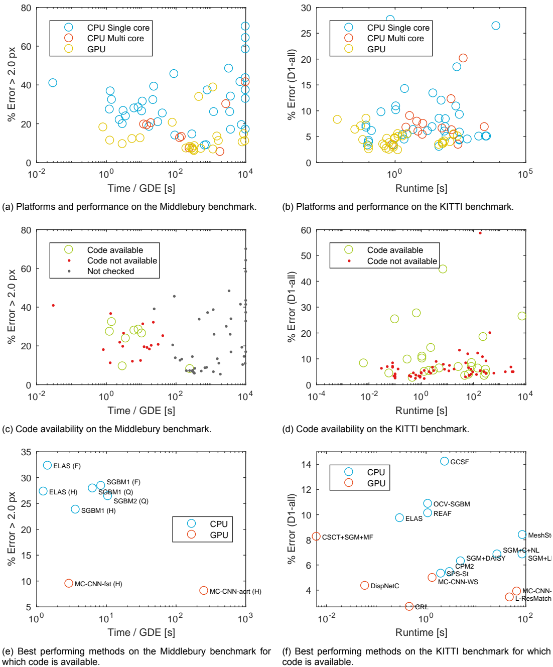
Figure 2.3: Scatterplots of accuracy versus runtime performance on the Middlebury and KITTI stereo vision benchmarks. Data obtained on 27/11/2017. a, b : Methods running on the GPU tend to perform better than those running on the CPU. On the Middlebury benchmark they perform better in terms of accuracy, while on the KITTI benchmark they also outperform CPU methods in terms of runtime – perhaps because runtime performance is more important for automotive applications than for the static pictures of Middlebury. c, d : While code is not available for every method, there are enough close-to-optimal algorithms for which source code has been published. e, f : These methods should be considered first when choosing a stereo vision algorithm, as they perform well and their code is publicly available. Popular choices are ELAS [18] and SGM/SGBM [23]; the latter is also included in OpenCV.
