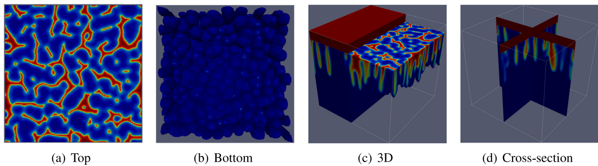
Fig. 9. Evolution of CO 2 fingers in the presence of a CTZ at 50 years. In (a), the CTZ zone saturated with CO 2 is removed for a better view; similarly, in (c), a threshold ([0.001, 0.0225]) is applied to illustrate the migration of CO 2 fingers inside the model.
