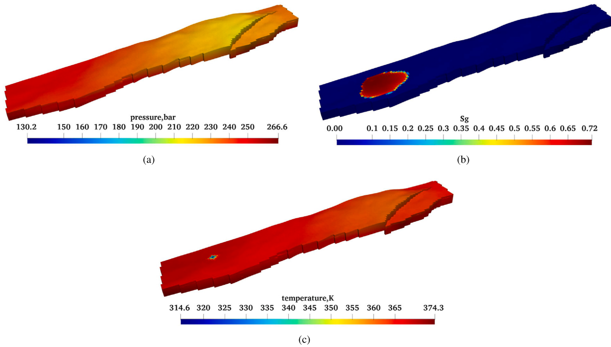
Fig. 11. Distribution of pressure, gas saturation and temperature after CO 2 injection.
