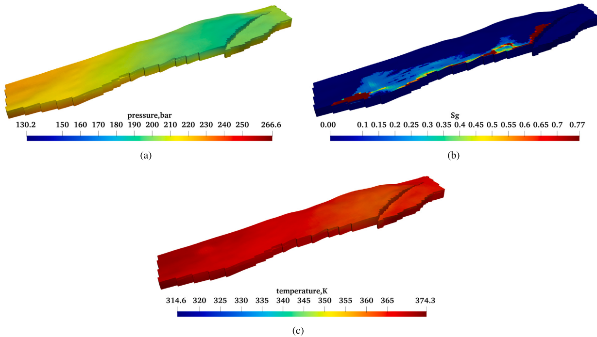
Fig. 12. Distribution of pressure, gas saturation and temperature in 100 years after CO 2 injection.
