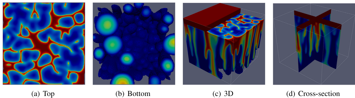
Fig. 10. Evolution of CO 2 fingers in the presence of a CTZ at 100 years. In (a), the CTZ zone saturated with CO 2 is removed for a better view; similarly, in (c), a threshold ([0.001, 0.0225]) is applied to illustrate the migration of CO 2 fingers inside the model.
