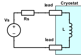
FIGURE 1. Topology 0: the power source directly connected to a HTS degaussing coil.
