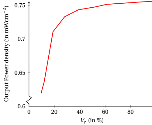
Figure 3.7: Solar cell power outputs for different electrode material volume fractions for the rear side of the cell.
