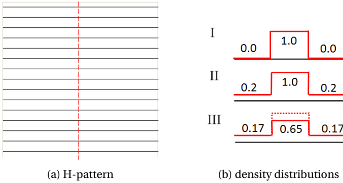
Figure 2.19: H-pattern and the density distribution corresponding to an electrode finger for 3 different cases.
