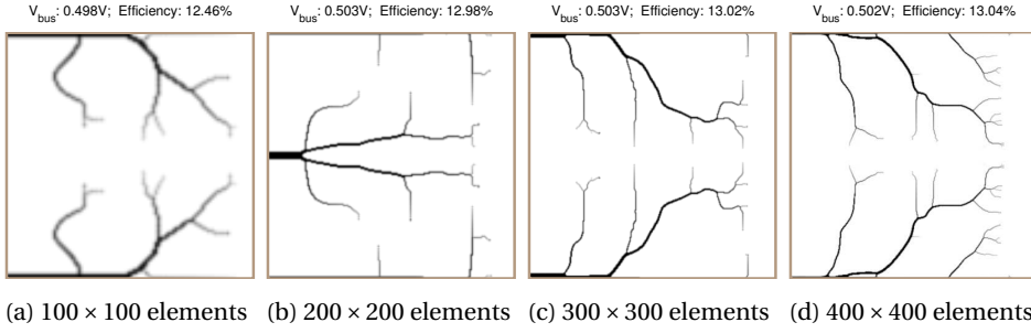
Figure 2.8: Front electrode patterns for side-contact solar cells with different mesh resolutions at constant value of r_{min} ( r_{min} = 1.5 element widths).
