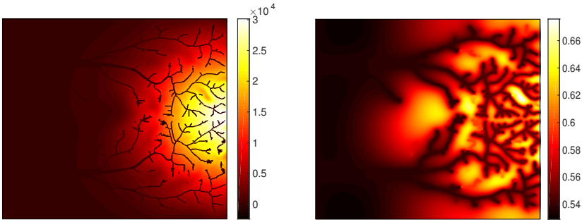
(b) Current density (in \text{Am}^{-2} )
