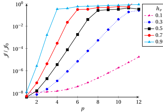
Figure 7.7: Compliance accuracy ( \mathcal{J}/\mathcal{J}_0 ) versus the shape function order ( p ) for different void-feature resolutions obtained using a single finite element (as shown in Fig. 7.6) comprising 10 \times 10 density voxels. Here, \mathcal{J} is the compliance obtained using the MTO setting, and \mathcal{J}_0 denotes the analytical solution.
