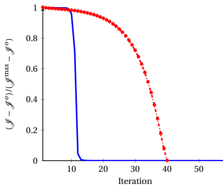
Figure 7.14: Normalized convergence plots of compliance objective values obtained for the axial load case shown in Fig. 7.4 using a homogeneous density field (red) and the density field shown in Fig. 7.12a (blue). For both the cases, r_{\min} is set to 3.6 voxels and material volume fraction is limited to 0.5. The domain is discretized using one finite element with p = 6 and comprises 8 \times 8 density voxels.
