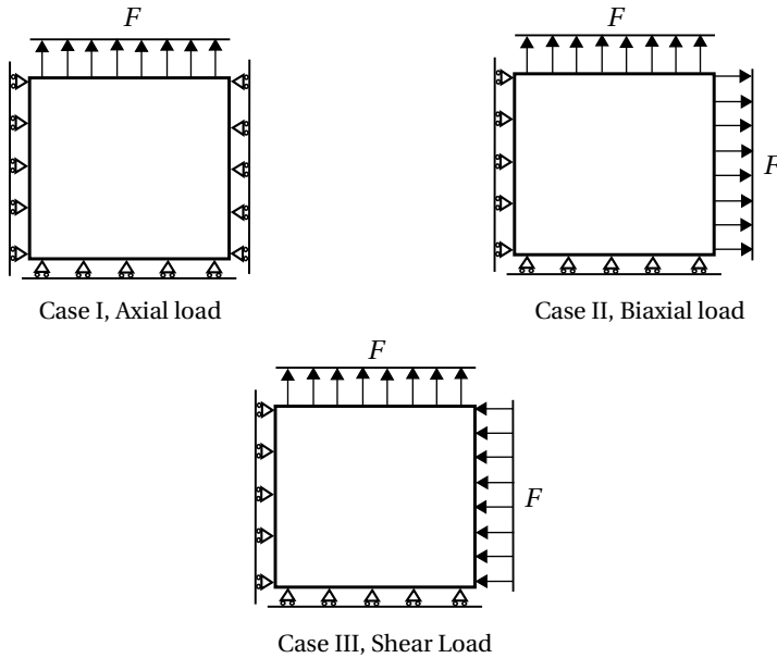
Figure 7.4: Numerical test cases with different loading conditions ( F = 1\text{Nm}^{-1} ). For modeling, the design domain for each case is discretized using a single finite element with shape functions of polynomial order 6, and 8 \times 8 design voxels are used.
