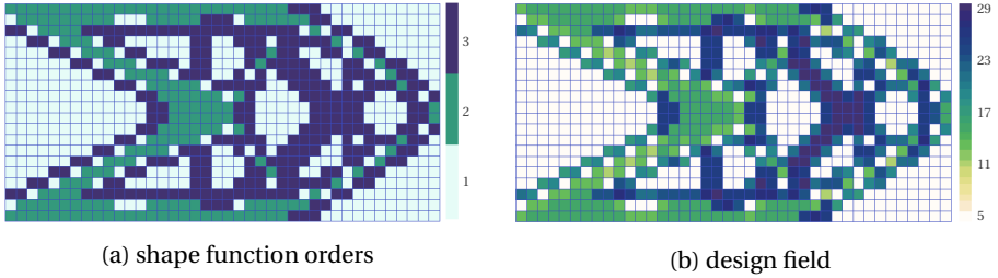
Figure 8.7: Distribution of polynomial orders of the shape functions (left) and the design field (right), showing the number of design points per MTO element, obtained from adaptive refinement (cycle 1) controlled by only density-based refinement indicator for a cantilever subjected to point load, as shown in Fig. 8.4a. The initial mesh comprises 40 \times 20 Q2 finite elements with 16 design points and 4 \times 4 density cells per element. The optimized design used for adaptive refinement is shown in Fig. 8.5.
