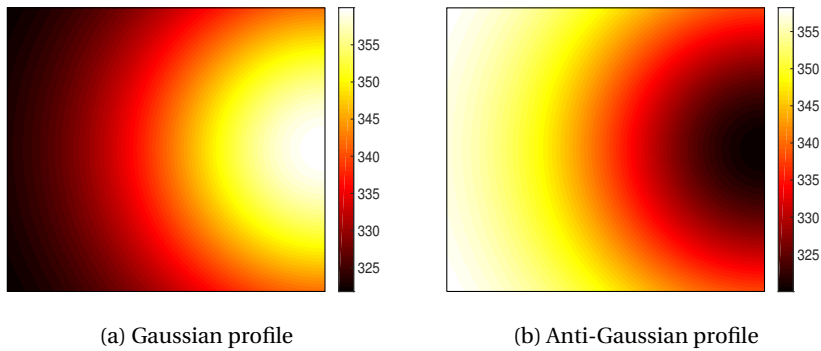
Figure 4.8: Non-uniform temperature profiles with base temperatures equal to 320 K. The temperature amplitude for both cases is set to 40 K deviation from the base temperature.
