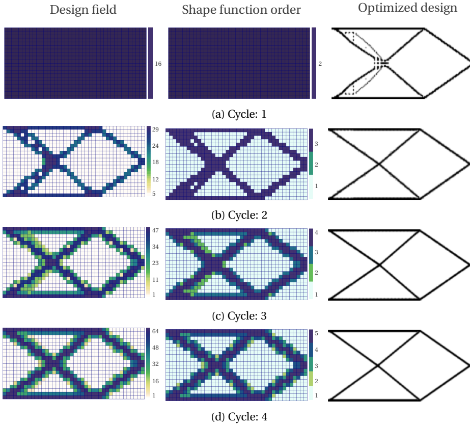
Figure 8.14: Optimized designs (right) and the respective shape function orders (middle) and design field (left) obtained for 4 cycles of dp -adaptive MTO run for a cantilever beam subjected to point load (Fig. 8.4a). The initial mesh is uniform and each element has shape functions of polynomial order 2 and 16 design points per element. The maximum allowed shape function order and number of design points are restricted to 5 and 64 per element, respectively.
