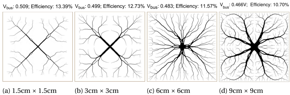
Figure 2.15: Optimized front electrode patterns for PUM solar cells of different sizes. The topology mesh for all the cases is same and comprises of 600 \times 600 elements.
