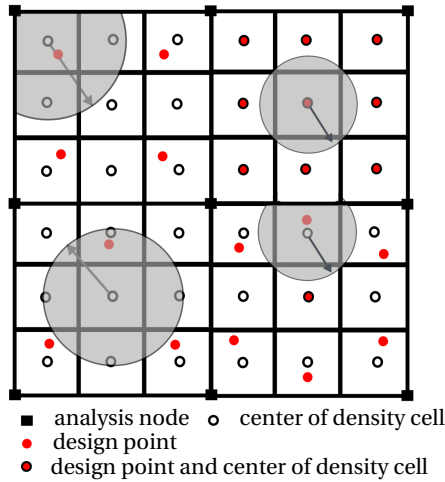
Figure 8.2: Schematic representation of projection P_1 illustrating the projection of density values from the design points in the design mesh to the centers of density cells of the background domain. Four projection regions are indicated in gray. Note that these projections are localized and operate on the design points and the density cell-centers of the same element. Here, the four MTO elements from top-left to bottom-right consist of 4, 9, 3 and 7 design points, respectively. The densities at the centers of the gray projection domains (denoted by ○) shown in each MTO element are computed from contributions of all design points (denoted by ●) of the same MTO element within its projection domain.
