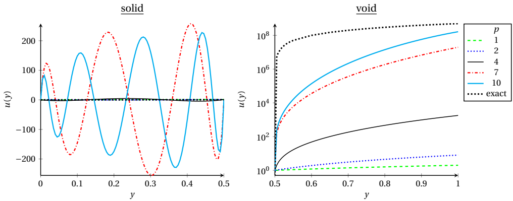
(b) Displacement fields in the solid (left) and void (right) parts. Note that the right-hand graph uses a log scale because of the large displacement differences.
