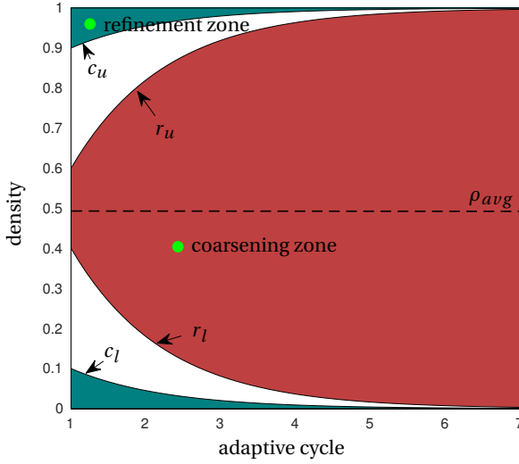
Figure 8.6: Bounds for the design refinement indicator as a function of the adaptive cycle [20].
