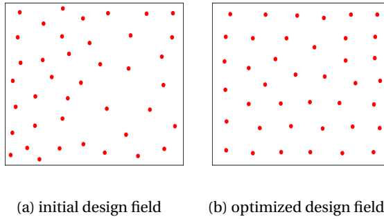
Figure 8.21: Distribution of 40 design points in a Q-type finite element obtained using k -means clustering.
