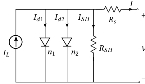
Figure 4.1: Equivalent electrical circuit diagram for a solar cell
