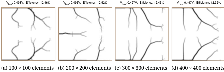
Figure 2.9: Front electrode patterns for side-contact solar cells with different mesh resolutions using mesh-independent density filter.
