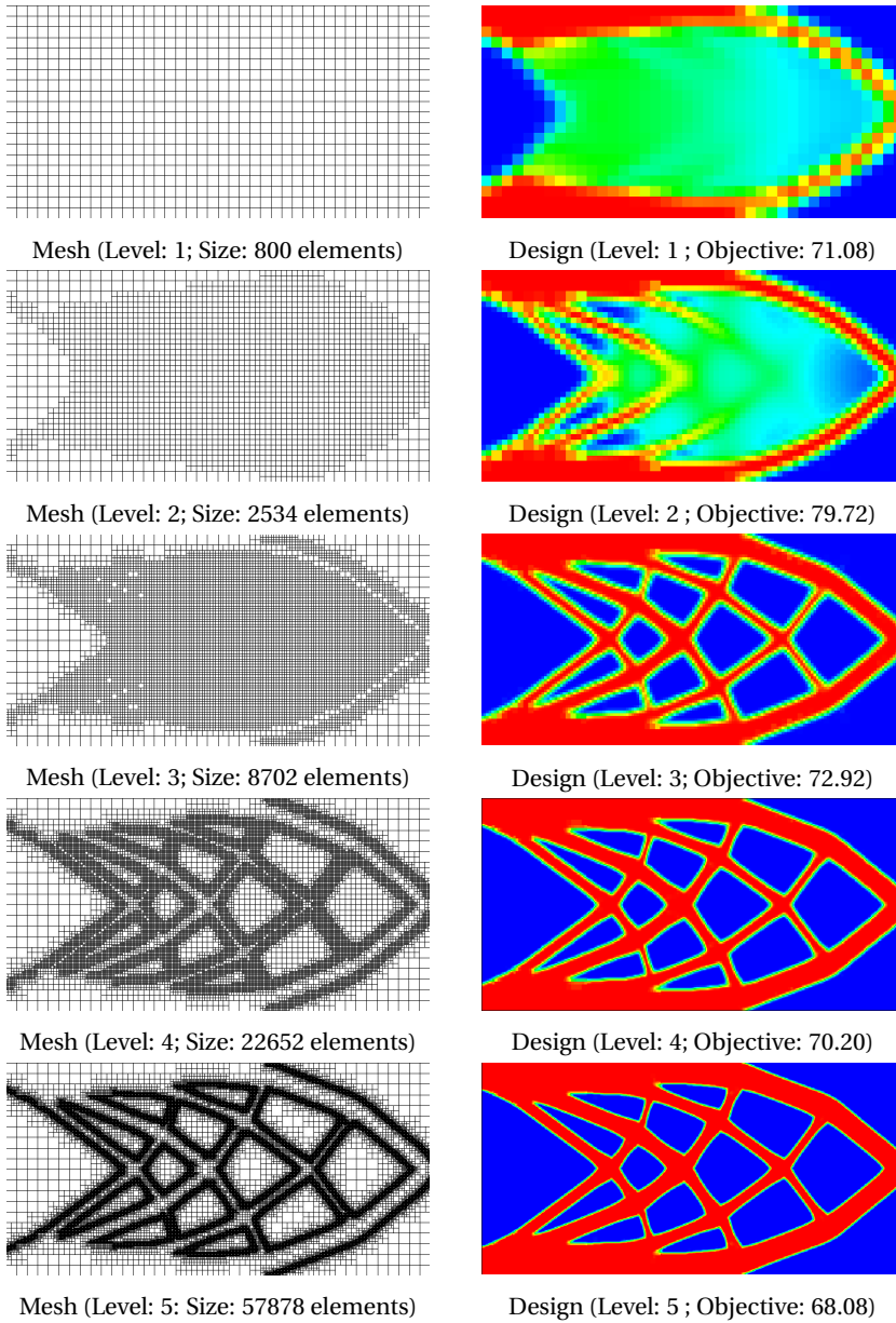
Figure 5.7: Cantilever example considering the proposed adaptive topology optimization scheme. It includes the adaptivity on the mesh and the filter radius and continuation of the penalization.
