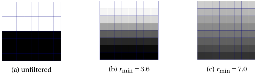
Figure 7.12: Unfiltered density field and its filtered versions obtained using density filters with r_{\min} equal to 3.6 and 7.0 voxels. The domain consists of 1 finite element with 8 \times 8 voxels.
