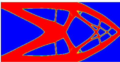
(a) Constant penalization (Objective: 69.38)
