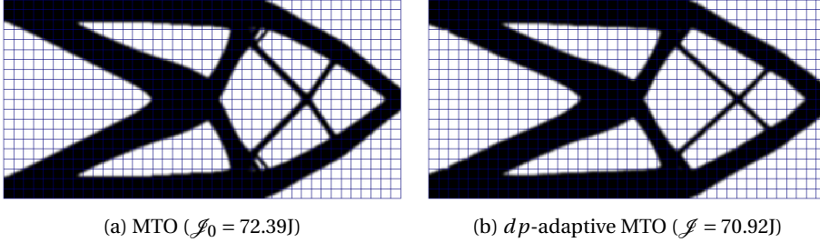
Figure 8.10: Optimized cantilever designs for the point load case shown in Fig. 8.4a, obtained using (a) a uniform MTO mesh and (b) dp -adaptive MTO approach. The maximum permissible material volume fraction is set to 0.45. A 4.5-fold speed-up as well as a superior objective value are obtained using dp -adaptivity. Additional information related to this test case is listed in Table 8.1.
