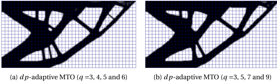
Figure 8.16: Optimized cantilever designs for the distributed-load case shown in Fig.8.9a, obtained using dp -adaptive MTO approach. For both the cases, adaptive penalization has been used. For the 4 cycles of the dp -adaptive MTO run, the values of q used have been reported in the sub-captions.
