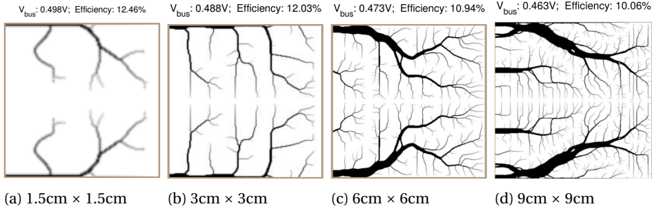
Figure 2.12: Optimized front electrode patterns for side-contact solar cells of different sizes. The mesh resolution for all the cases is same and the size of an element in all the cases is 0.015\text{cm} \times 0.015\text{cm} .
