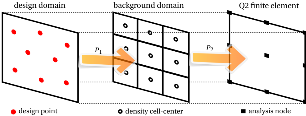
Figure 8.1: Schematic representation of a Q2/d8 MTO element comprising 3 linked overlapping domains. These domains represent a design domain with 8 design points (left) and a Q2 finite element (right), with a background distribution of 3 \times 3 density cells (middle). Here, P_1 and P_2 denote the projections from the design to background domain and from background domain to the finite element, respectively. The design points are distributed in the domain using a variant of the k -means clustering approach (Appendix 8.A).
