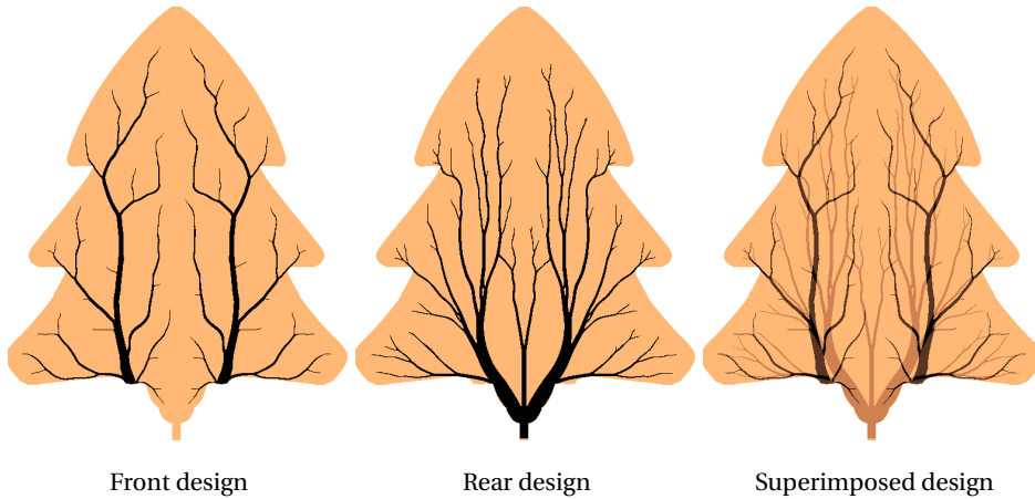
Figure 3.6: Fully optimized metallization patterns for a solar cell with Christmas tree shape.
