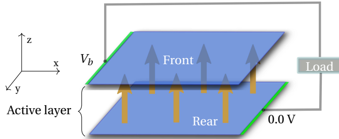
Figure 3.1: Schematic diagram of a solar cell model with front and rear conductive surfaces. The voltage difference between the front and rear sides, combined with the illumination level, controls the current density across any point in the semiconductor layer.
