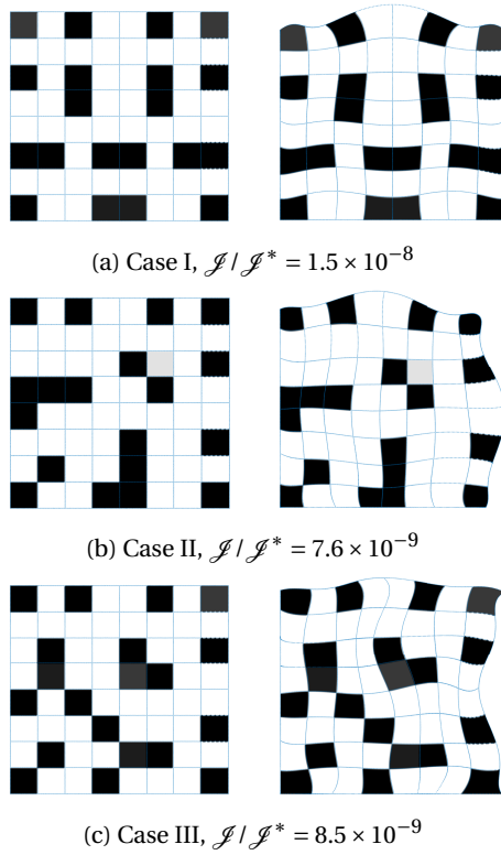
Figure 7.5: Optimized designs (left) and respective deformed shapes (right, scaled for visualization) under various loading conditions obtained for a single finite element obtained using an MTO scheme with p = 6 and 8 \times 8 voxels.
