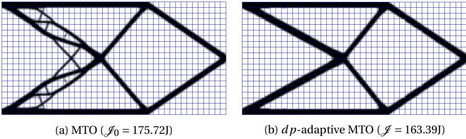
Figure 8.12: Optimized cantilever designs for the point load case shown in Fig. 8.4a, obtained using a uniform MTO mesh (left) and dp -adaptive MTO approach (right). The maximum permissible material volume fraction is set to 0.20. A speed-up of 8.3 times is obtained using dp -adaptivity. Additional information related to this test case is listed in Table 8.1.
