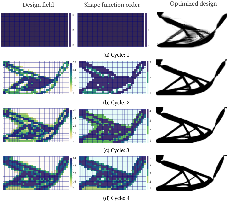
Figure 8.19: Optimized designs (right), and the respective shape function orders (middle) and design field (left) obtained for 4 cycles of a dp -adaptive MTO run for the force inverter problem shown in Fig. 8.9b. The initial mesh is uniform and each element comprises shape functions of polynomial order 2 and 16 design points per element. The maximum allowed order of the shape functions and number of design points are restricted to 5 and 64 per element, respectively.
