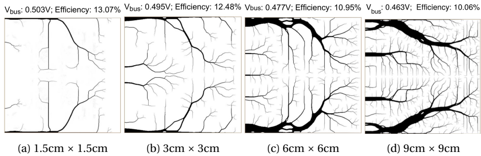
Figure 2.14: Optimized front electrode patterns for side-contact solar cells of different sizes. The topology mesh for all the cases is same and comprises of 600 \times 600 elements.
