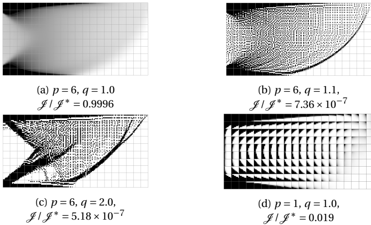
Figure 7.10: Optimized designs for a cantilever beam subjected to a distributed load obtained using various penalization powers q in the modified SIMP formulation. The domain consists of 20 \times 10 finite elements with 8 \times 8 voxels per element.
