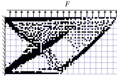
Figure 7.1: Design obtained in MTO compliance minimization of a cantilever beam subjected to a distributed load. The domain is discretized using 20 \times 10 finite elements with shape functions of polynomial degree 3 and 4 \times 4 design voxels per element. A composite integration scheme with 4 th order Gauss quadrature rule is used in each voxel.
