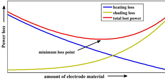
Figure 2.5: Qualitative effect of series resistance and shading on total power lost in a solar cell, in relation to the amount of front electrode material.
