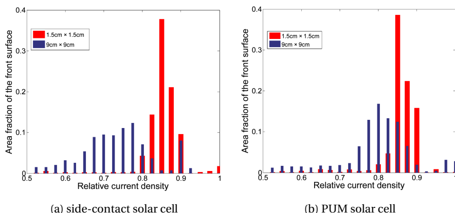
Figure 2.17: Area fractions of the front surface corresponding to different values of relative current density. Relative current density here, is the actual current density value normalized by the maximum current density value on the front surface.
