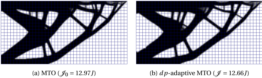
Figure 8.15: Optimized cantilever designs for the distributed-load case shown in Fig.8.9a, obtained using a uniform MTO mesh (left) and dp -adaptive MTO approach (right). A 4.6-fold speed-up is obtained using dp -adaptivity.
