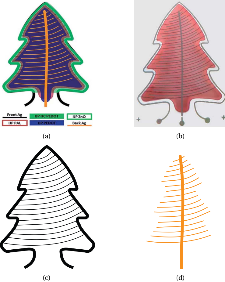
Figure 3.2: Christmas tree shaped free-form solar cell, (a) schematic diagram showing the layout of different printed layers [8] (b) photograph of the solar cell fabricated using inkjet printing [8] (c) modeled front side metallization design and (d) modeled rear side metallization design.
