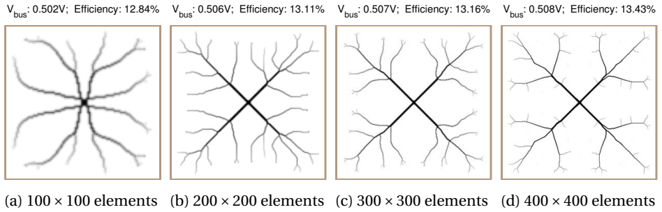
Figure 2.10: Front electrode patterns for PUM solar cells with different mesh resolutions at constant value of r_{min} ( r_{min} = 1.5 element widths).
