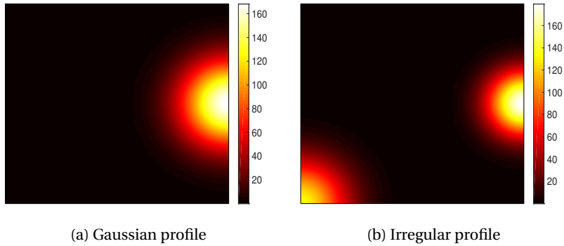
Figure 4.7: Non-uniform illumination profiles with an average illumination of 12 suns (1 sun = 1000 \text{ Wm}^{-2} ). For the Gaussian profile, A_0 is equal to 15 and for the irregular profile A_0 values are 15 and 20 for the two Gaussian distributions.
