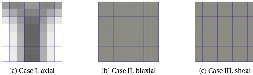
Figure 7.16: Optimized designs for the three elementary test cases shown in Fig. 7.6 obtained using a filter radius of 2.6 voxels. The domain consists of 1 finite element with 8 \times 8 voxels and shape functions of polynomial degree 6.
