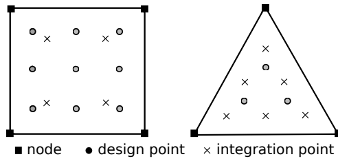
Figure 6.1: Q4 element (left) with 9 design points and 4 integration points ( Q4/n4/d9 ) and a T3 element (right) with 3 design points and 6 integration points ( T3/n6/d3 ).
