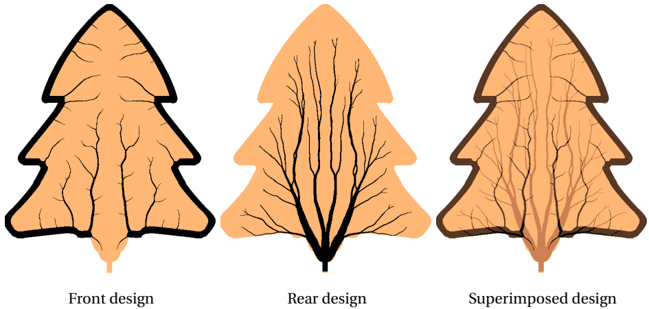
Figure 3.5: Optimized metallization patterns with a pre-defined perimeter electrode for the front side for a solar cell with Christmas tree shape.
