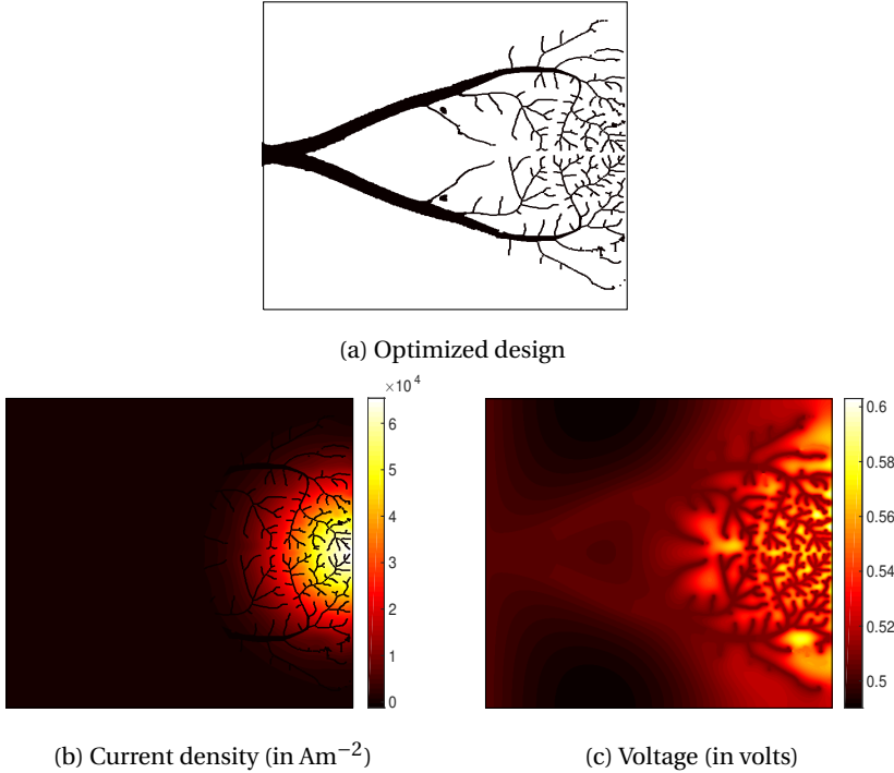
Figure 4.14: Optimized design and the current density and voltage distributions for the front side of a solar cell under a Gaussian illumination of an average intensity of 12 suns ( A_0 = 15 ) and a Gaussian temperature profile with base temperature of 320 K and temperature amplitude equal to 40 K. The optimal busbar potential V_b and efficiency \eta values are 0.503 volts and 15.033%, respectively.
