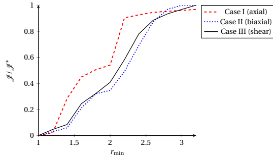
Figure 7.15: Compliance accuracy \mathcal{J}/\mathcal{J}^* for various filter radii r_{\min} obtained for the three test cases presented in Fig. 7.4. For all the cases, a single finite element is used with shape functions of polynomial order 6 and 8 \times 8 design voxels.
