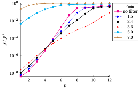
Figure 7.11: Compliance accuracy \mathcal{J}/\mathcal{J}^* versus the shape function order p for various filter radii r_{\min} (in terms of voxel-length) obtained using a single finite element comprising 8 \times 8 design voxels. The unfiltered density field consists of solid and void parts in equal proportions.
