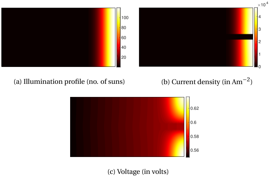
Figure 4.5: Non-uniform illumination profile with an average illumination of 12 suns and peak illumination ratio of 10 and the out-of-plane current density and voltage distributions observed in one cell element (1 sun = 1000 \text{ Wm}^{-2} ).
