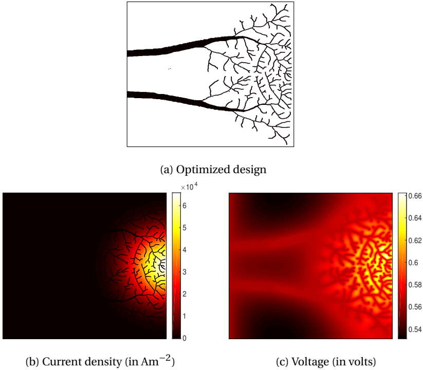
Figure 4.10: Optimized design and the current density and voltage distributions for the front side of a solar cell under a Gaussian illumination of an average intensity of 12 suns ( A_0 = 15 ). A uniform temperature profile is chosen with base temperature set to 320 K. The optimal busbar potential V_b and efficiency \eta values are 0.562 volts and 17.271%, respectively.
