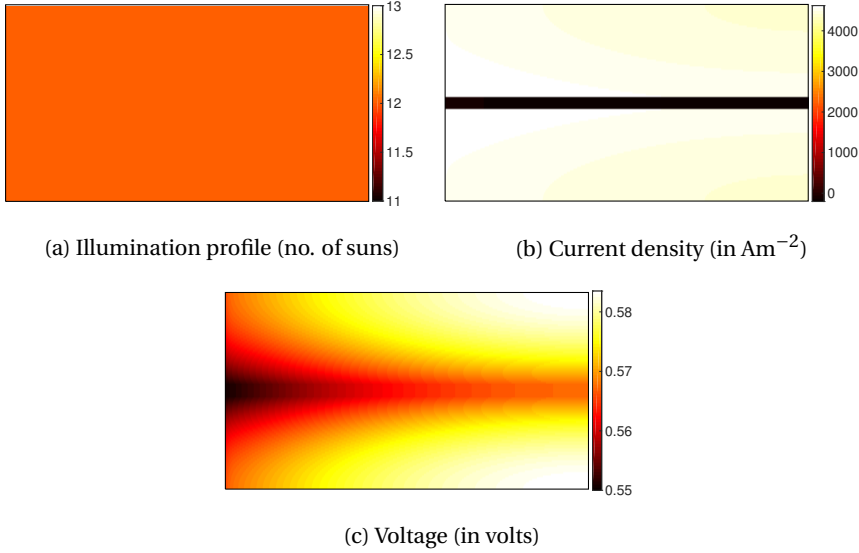
Figure 4.4: Uniform illumination profile for 12 suns and the out-of-plane current density and voltage distributions observed in one cell element (1 sun = 1000 \text{ Wm}^{-2} ).
