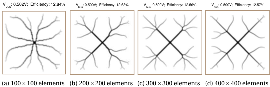
Figure 2.11: Front electrode patterns for PUM solar cells with different mesh resolutions using mesh-independent density filter.
