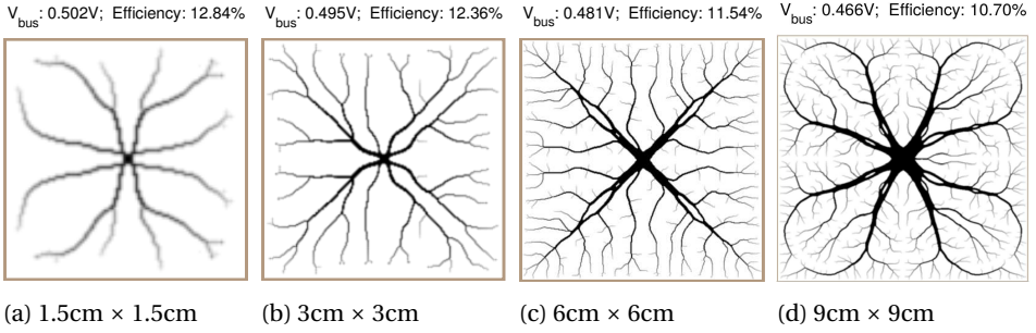
Figure 2.13: Optimized front electrode patterns for PUM solar cells of different sizes. The mesh resolution for all the cases is same and the size of an element in all the cases is 0.015\text{cm} \times 0.015\text{cm} .
