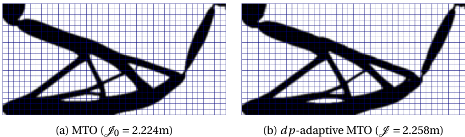
Figure 8.18: Optimized cantilever designs for the force inverter problem shown in Fig.8.9b, obtained using a uniform MTO mesh (left) and dp -adaptive MTO approach (right). A speed-up of 6.2 folds is obtained using dp -adaptivity.
