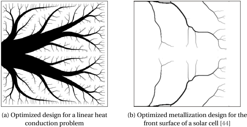
Figure 8.20: Optimized designs obtained using the traditional TO approach on a mesh of 400 \times 400 finite elements, with R set to 1.5 elements. The two cases refer to (a) linear heat conduction problem with V_0 set to 0.3, and (b) nonlinear electrical conduction problem [44].
