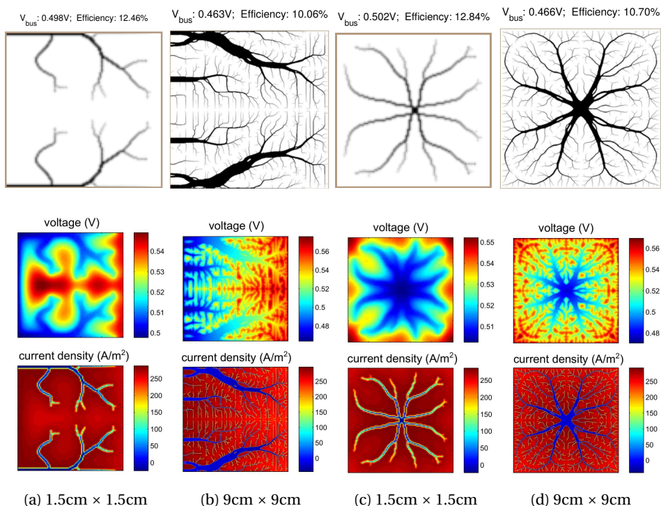
Figure 2.16: Front electrode patterns, out-of-plane current density distributions and voltage distributions for side-contact (a and b) and PUM (c and d) solar cells obtained using topology optimization.
