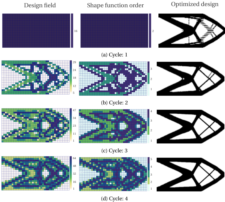
Figure 8.11: Optimized designs (right), and the respective shape function orders (middle) and design field (left) obtained for 4 cycles of dp -adaptive MTO run for a cantilever beam subjected to point load (Fig. 8.4a). The initial mesh is uniform and each element has shape functions of polynomial order 2 and 16 design points per element. The maximum allowed shape function order and number of design points are restricted to 5 and 64 per element, respectively.
