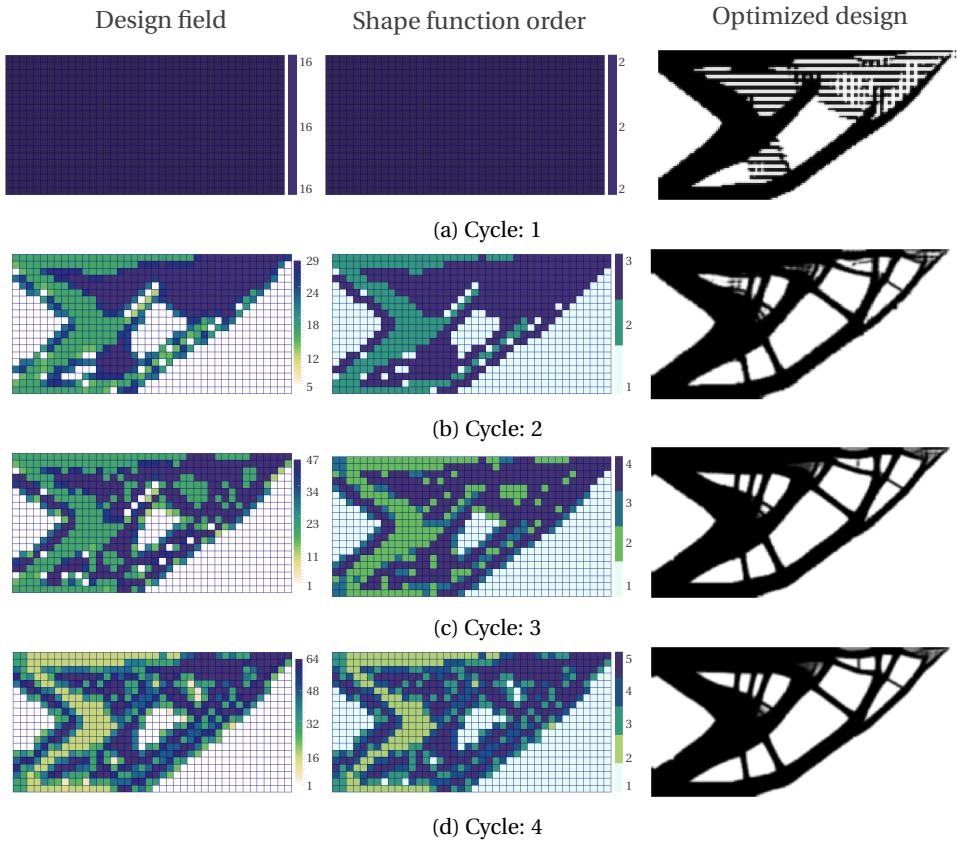
Figure 8.17: Optimized designs (right), and the respective shape function orders (middle) and design field (left) obtained for 4 cycles of dp -adaptive MTO run for a cantilever beam subjected to distributed load (Fig. 8.9a). The domain has been discretized using 40 \times 20 quadrilateral finite elements ( r = 0.3h ). The initial mesh is uniform and each element comprises shape functions of polynomial order 2 and 16 design points per element. The maximum allowed shape function order and number of design points are restricted to 5 and 64 per element, respectively.
