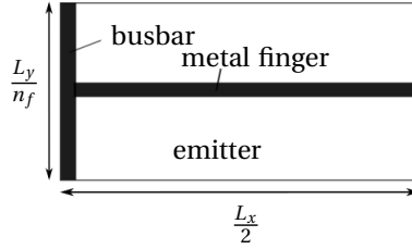
Figure 4.3: The cell element used for modeling purposes. Here, L_x and L_y are the cell lengths along x- and y-directions and n_f denotes the number of metal fingers.
