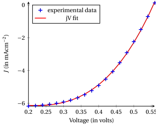
Figure 3.3: J-V data measured for a small device ( 0.04 \text{ cm}^2 ) and the fitted J-V curve (obtained using a cubic polynomial) for the OPV solar cell used in this study.
