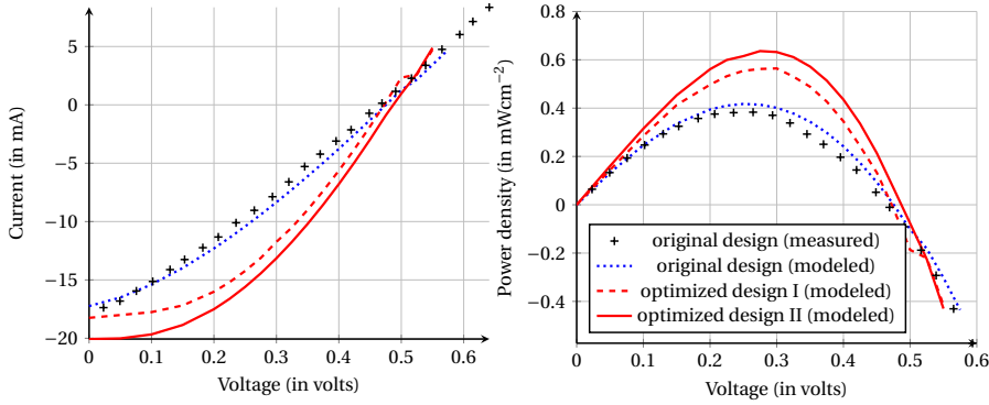
Figure 3.4: I-V and P-V curves for the modeled solar cell with Christmas tree shape.
