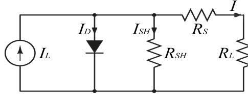
Figure 2.2: Equivalent electrical circuit for a solar cell [23].
