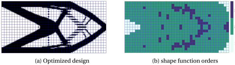
Figure 8.5: Optimized design (left), and the distribution of shape function orders (right) obtained from adaptive refinement controlled by only analysis-based refinement indicator for a cantilever subjected to point load, as shown in Fig. 8.4a. The optimized design clearly shows typical artefacts (QR-patterns) of disconnected structural features. The initial mesh comprises 40 \times 20 Q2 finite elements with 16 design points and 4 \times 4 density cells per element. Based on the ranking of analysis-based refinement indicator values, top 10% and bottom 5% of the MTO elements have been chosen for refinement and coarsening, respectively.
