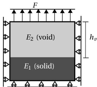
Figure 7.6: An axially loaded finite element ( F = 1\text{Nm}^{-1} ) filled with solid and void parts.
