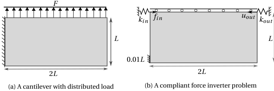
Figure 8.9: Problem domains and boundary conditions for a cantilever beam subjected to distributed load (left) and a force inverter (right). Here, L = 1 m, F = \frac{0.5N}{L} , k_{in} = 1 \text{ Nm}^{-1} , k_{out} = 0.001 \text{ Nm}^{-1} and f_{in} = 1 N.
