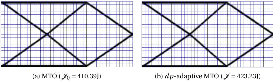
Figure 8.13: Optimized cantilever designs for the point load case shown in Fig. 8.4a, obtained using a uniform MTO mesh (left) and dp -adaptive MTO approach (right). The maximum permissible material volume fraction is set to 0.10. A 10-fold speed-up is obtained using dp -adaptivity. Additional information related to this test case is listed in Table 8.1.
