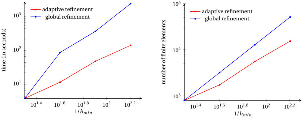
Figure 5.5: (a) Computational time (in seconds) and (b) number of elements needed to achieve a desired design resolution. The design resolution is characterized by the inverse of the minimum element size ( 1/h_{min} ).
