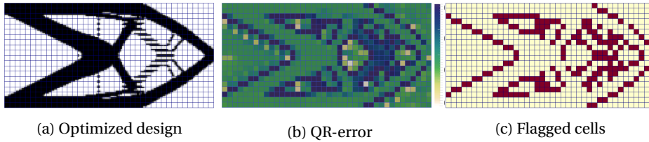
Figure 8.8: (a) Optimized design obtained after first cycle of dp -adaptive MTO run for a cantilever subjected to point load (Fig. 8.4a), (b) corresponding QR-error distribution plot obtained during the first adaptive cycle, and (c) domain showing the elements flagged for refinement using the QR-indicator. To avoid excessive refinement, only cells with error value larger than 0.9 have been flagged for refinement. The initial mesh comprises 40 \times 20 Q2 finite elements with 16 design points and 4 \times 4 density cells per element.
