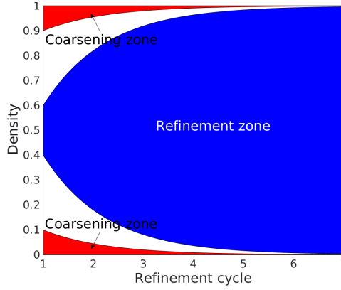
Figure 5.1: Bounds for the mesh refinement indicator as a function of the refinement cycle
