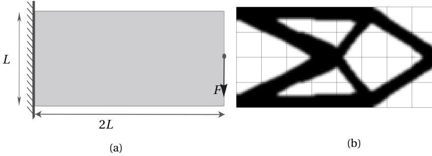
Figure 8.4: (a) Example of a cantilever beam subjected to a point load, and (b) the optimized design obtained using MTO for compliance minimization using 8 \times 4 Q10/d225 elements and R = 0.13h . Here, Q10/d225 refers to a quadrilateral finite element with shape functions of polynomial order 10 and 225 design points.
