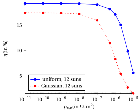
Figure 4.6: Effect of resistivity of the ohmic contact between the emitter and electrode, \rho_{c,e} , on the efficiency of a solar cell.
