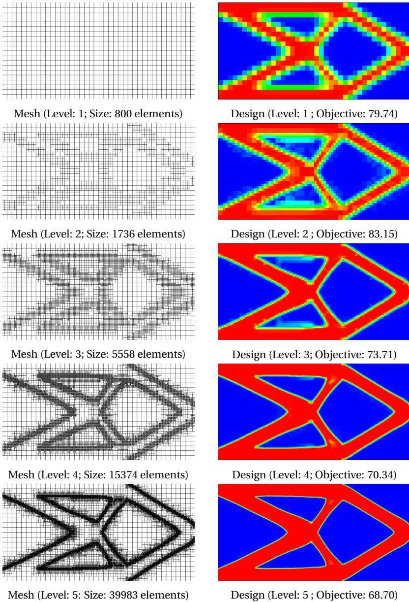
Figure 5.4: Cantilever example considering the adaptive mesh refinement and filter radius.
