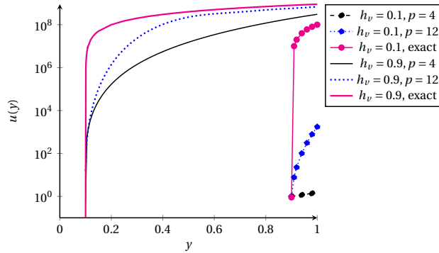
Figure 7.9: Displacement field u(y) (on a log scale) in the void region for the 1D bar example shown in Fig. 7.8a. The log scale has been used due to large differences in the displacements for different values of p .
