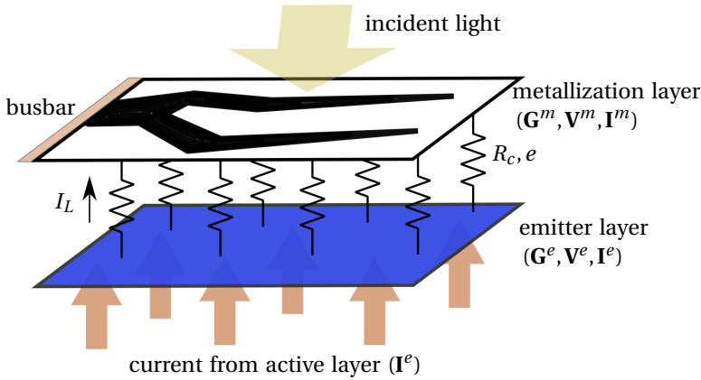
Figure 4.2: A two-layer finite element model of the front surface of a solar cell. Layer 1 comprises the emitter material and layer 2 consists of electrode material parts and void parts. Each node of the emitter layer is connected to the respective node in the metal layer with a resistor (contact resistance R_{c,e} ).
