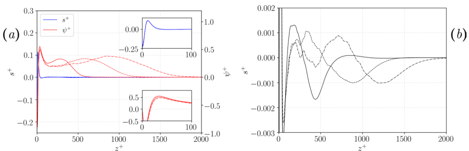
Fig. 7 a Extended source s^+(z^+) and spatial flux \psi^+(z^+) of turbulent kinetic energy for three different evolution times corresponding to Re_\tau = 500 (solid), 1000 (dashed) and 1500 (dashed dotted). The two insets report an enlarged view of the near-wall behaviour. b Enlarged view of the second-outer source of turbulent kinetic energy
