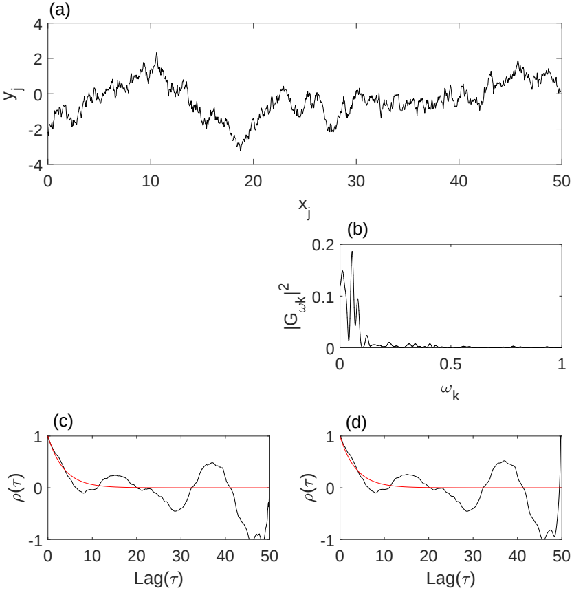
Figure 3.4: Example auto-correlation functions derived from generated data. (a) generated data based on Markov auto correlation with \theta = 5 , (b) power spectrum density function |G(\omega_k)|^2 , (c) auto-correlation function using Equations (3.3, 3.6), and (d) auto-correlation function using Equations (3.7, 3.8).
