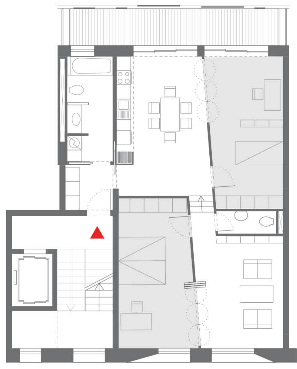
TYPOLOGY: LIVING ONE living 93 sqm scale 1:100
