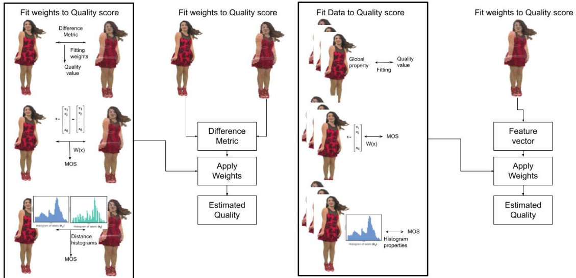
Figure 3.1: Process of fitting Full-Reference versus the process of fitting No-Reference metrics
