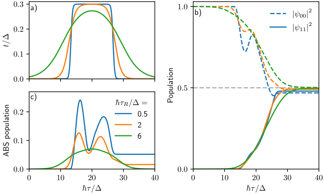
Figure 3: Time-dependent simulation of pairing gate \mathcal{U}_3 acting on an initial vacuum state with different pulse rise time \tau_R profiles. The vacuum population is |\psi_{00}|^2 whereas the double occupation population (with middle dot unoccupied) is |\psi_{11}|^2 . Longer pulses (a) result in a smoother transient population profile (b) and less leakage into the middle ABS state (c). The configuration is the spin-antiparallel with finite Zeeman field within the middle dot B/\Delta = 0.2 and symmetric spin-orbit precession \theta_L = \theta_R = \pi/8 .
