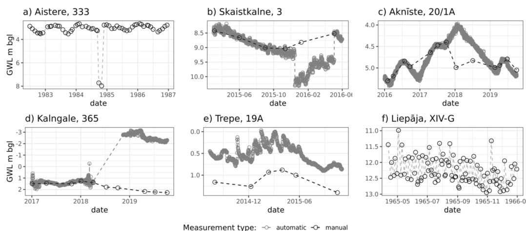
Fig. 5. Representative examples of groundwater level (GWL) time series where problems caused by data recordings and measurements were identified (title represent station name and well number).
