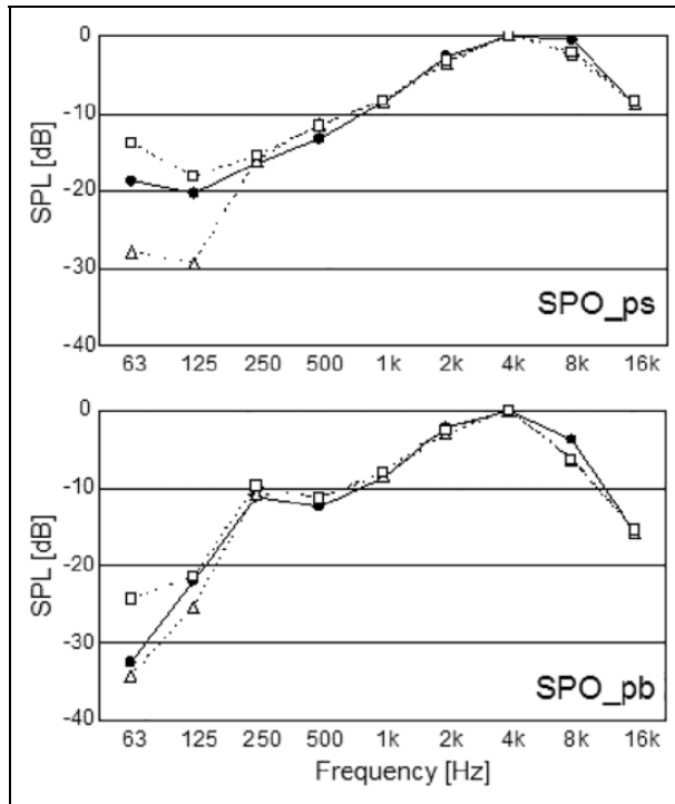
Figure 6. SPL as a function of band frequency: real IR (●), virtual IR by single stereo-dipole (Δ) and virtual IR by dual stereo-dipole (□), Spoletto 2/2.
