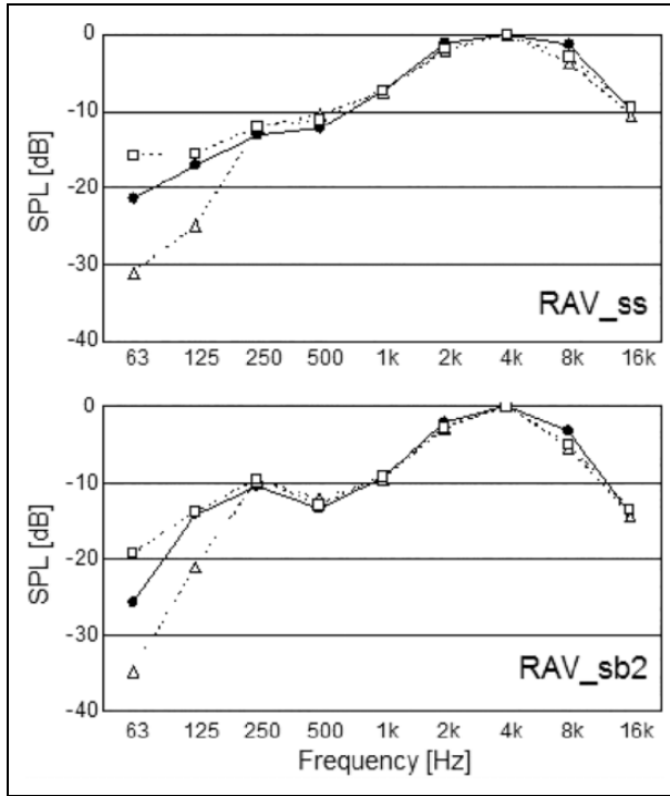
Figure 7. SPL as a function of band frequency: real IR (●), virtual IR by single stereo-dipole (△) and virtual IR by dual stereo-dipole (□), Ravenna 1/2.
