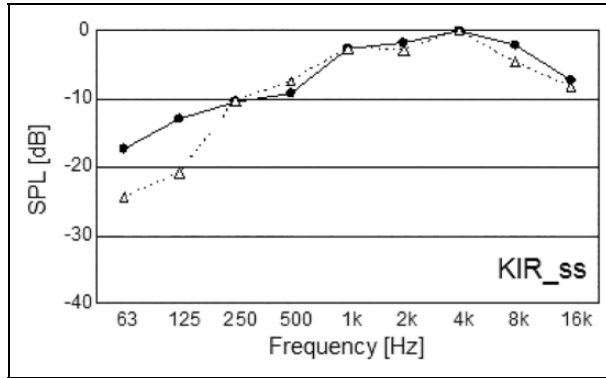
Figure 9. SPL as a function of band frequency: real IR (●) and virtual IR by single stereo-dipole, Kagoshima.
