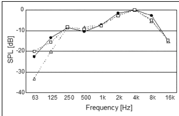
Figure 8. SPL as a function of band frequency: real IR (●), virtual IR by single stereo-dipole (△) and virtual IR by dual stereo-dipole (□), Ravenna 2/2.
