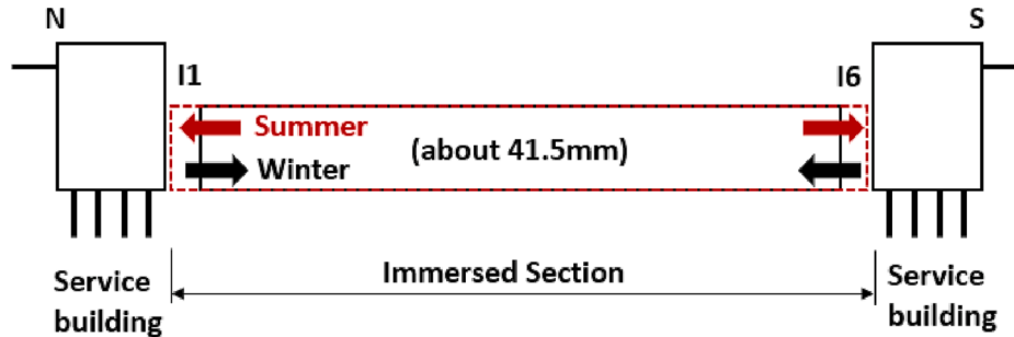
Fig. 19. Longitudinal expansion and contraction deformation of Heinenoordtunnel.
