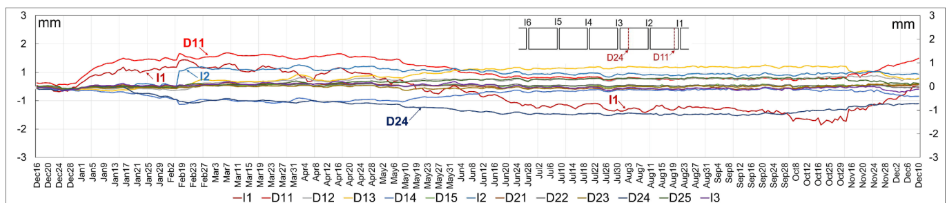
Fig. 20. Measured uneven settlement of 13 joints (full-year period).
