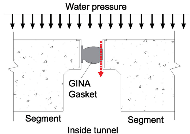
Fig. 23. Potential leakage risk due to large joint opening.
