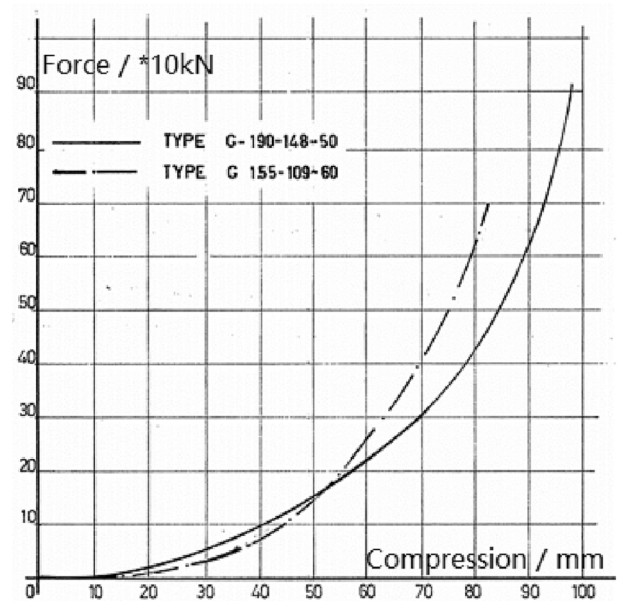
Fig. 24. Compression behavior of GINA gasket.
