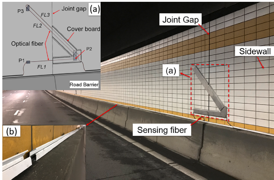
Fig. 10. Field fiber sensor installation in the Heinenoordtunnel:(a) Sensor layout at joint;(b) Loose fiber cable in PVC duct.
