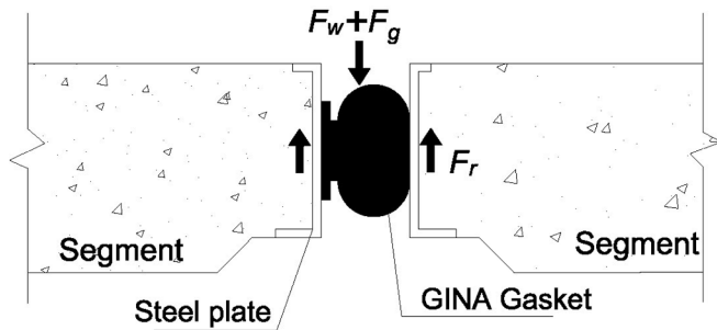
Fig. 25. Force Equilibrium on GINA gasket at immersion joint.
