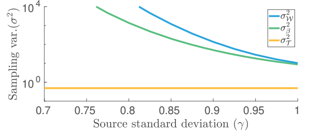
Fig. 4. Sampling variance of the target (yellow, \sigma_{\mathcal{T}}^2 ), the importance-weighted (blue, \sigma_{\mathcal{W}}^2 ) and the controlled importance-weighted (green, \sigma_{\beta}^2 ) risk estimators as a function of \gamma in the example setting.
