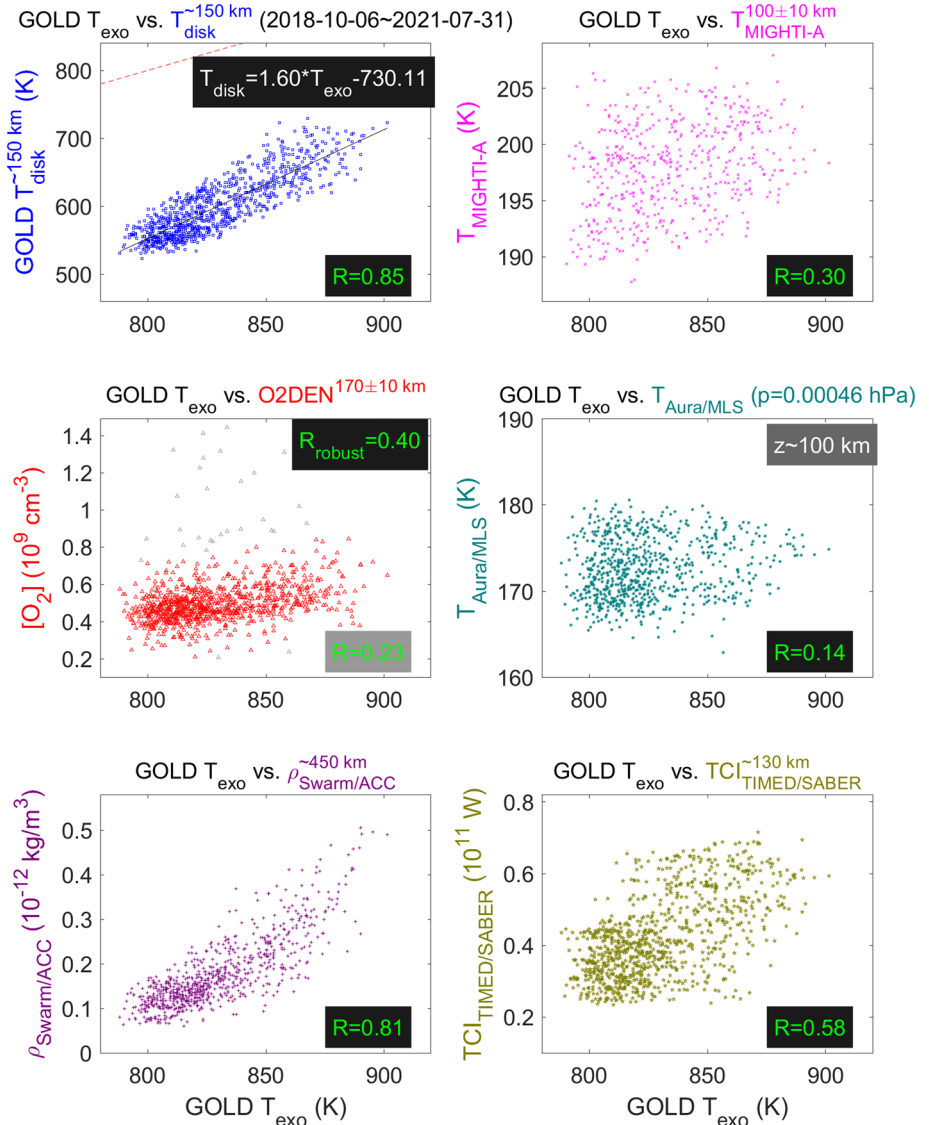
Figure 6. Scatterplots of GOLD T_{\text{exo}} with various data sets retrieved from GOLD and other LEO satellites: (a) GOLD T_{\text{disk}} relevant to altitudes of \sim 150 \text{ km} , (b) GOLD \text{O}_2 density relevant to altitudes of \sim 170 \text{ km} , (c) thermospheric mass density at altitudes of \sim 450 \text{ km} measured by Swarm-Charlie, (d) neutral temperature at altitudes of \sim 100 \text{ km} measured by ICON/MIGHTI-A, (e) neutral temperature at pressure level of 0.00046 \text{ hPa} ( \sim 100 \text{ km} ; see Waters et al., 2006, Figure 2) measured by Aura/MLS, and (f) Thermosphere Climate Index (TCI) deduced from the TIMED/SABER measurements around altitudes of 130 \text{ km} . The red dashed line in panel a represents the line of one-to-one correspondence (i.e., T_{\text{exo}} = T_{\text{disk}} ). The black solid line in panel a represents the polynomial fit, whose equation is annotated within the panel.
