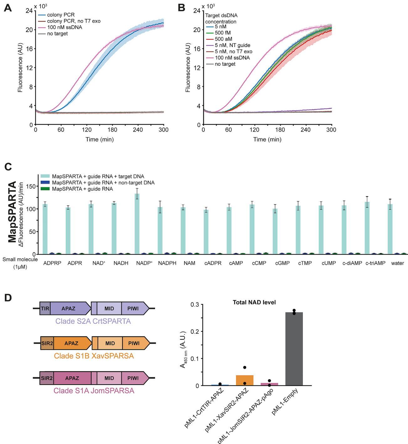
Figure S7. SPARTA can be used to detect dsDNA, and SPARSA systems degrade \text{NAD}^+ in vivo , related to Figure 7
