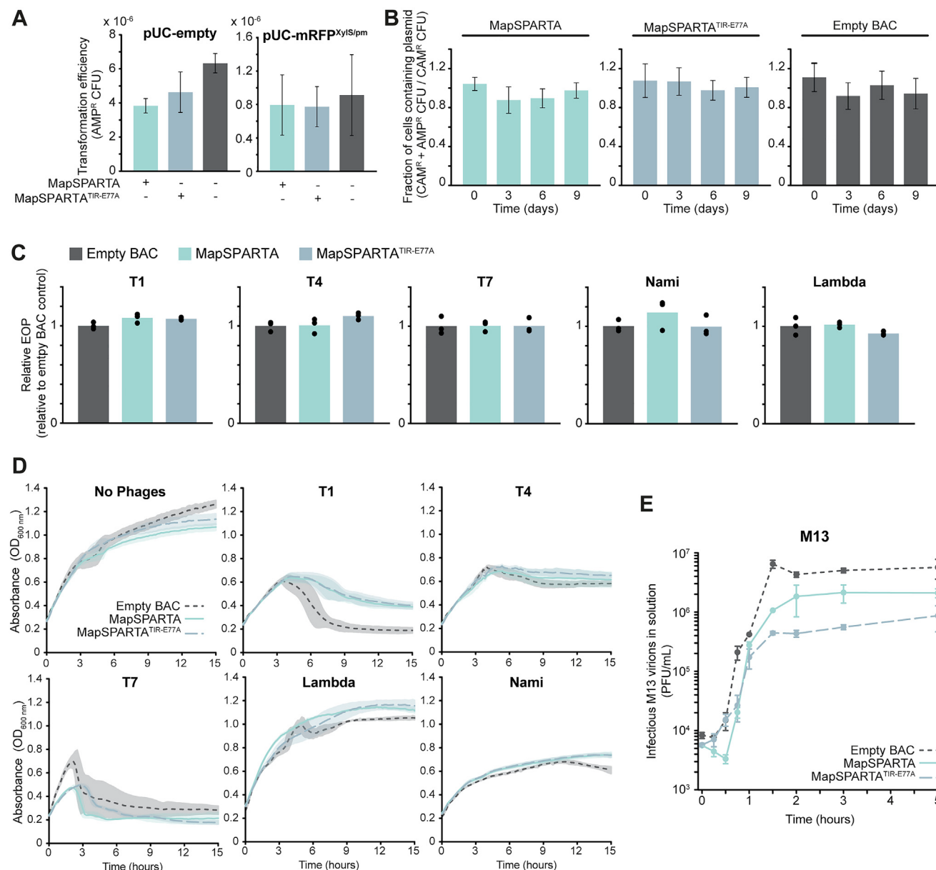
Figure S6. Effect of SPARTA on plasmid DNA and bacteriophages, related to Figure 6
