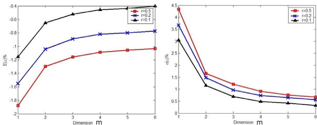
Figure 4. The scaling with dimensionality, m , of standard deviation of relative error, \epsilon , for of the quadrature-based method when applied to separable functions.
