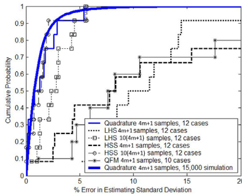
Figure 8. Empirical cumulative density functions based on the set of case studies. The model-based cumulative density functions of the 4m + 1 quadrature technique is provided for comparison.
