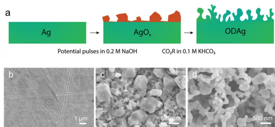
Figure 3.1. (a) Fabrication scheme of oxide-derived silver (ODAg), silver is denoted by green, silver oxide by dark orange. SEM images show how the surface morphology changes drastically when (b) silver is (c) oxidised to AgO x and (d) reduced to form ODAg.
