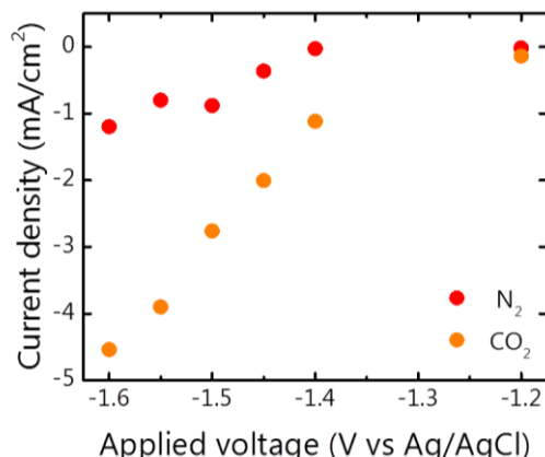
Figure 2.2. The average current density measured during the ATR-FTIR experiments at different potentials under both \text{N}_2 (red) and \text{CO}_2 (orange) flush.
