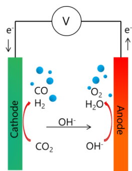
Figure 1.4. Schematic drawing of the electrochemical reduction of \text{CO}_2 to \text{CO} . The oxidation reaction of hydroxide ( \text{OH}^- ) into oxygen and water, and the unwanted side reaction forming hydrogen are also presented.
