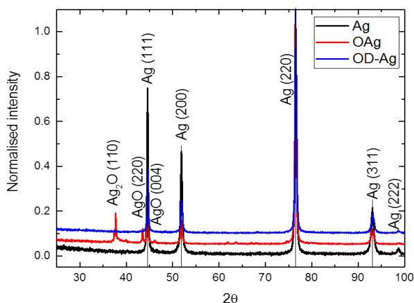
Figure B3. XRD patterns measured in Bragg-Brentano configuration of Ag, \text{AgO}_x and OD-Ag, showing the \text{Ag}_2\text{O} and AgO XRD reflections in the \text{AgO}_x sample. NB the XRD instrument was equipped with a cobalt source, resulting in a different 2\theta pattern compared to the GIXRD patterns.
