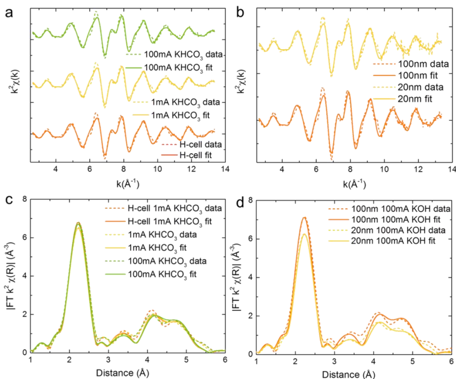
Figure 4.2. k^2 -weighted EXAFS data and fits of (a) several copper samples in a 1M \text{KHCO}_3 electrolyte: a Cu GDE at 1 mA/cm 2 in an H-cell configuration (orange) and in GDE configuration (yellow). And a sample at 100 mA/cm 2 (green). (b) Comparison between 100 nm (orange) and 20 nm (yellow) Cu films on GDEs at 100 mA/cm 2 in 1M KOH. (c) and (d) k^2 -weighted Fourier transformed EXAFS data of the spectra shown in (a) and (b) respectively. Note that the 1mA and 100mA labels in the figures correspond to 1 and 100 mA/cm 2 current density.
