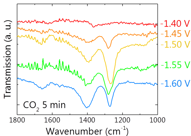
Figure A6. ATR transmission spectra in \text{CO}_2 0.1 M KCl electrolyte at different potentials 5 min after the \text{CO}_2 purge was turned on.
