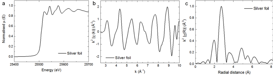
Figure 1.10. (a) Normalised absorption coefficient \mu(E) , (b) k^2 -weighted \chi(k) and (c) the Fourier transformed k^2 -weighted \chi(k) of a silver foil.
