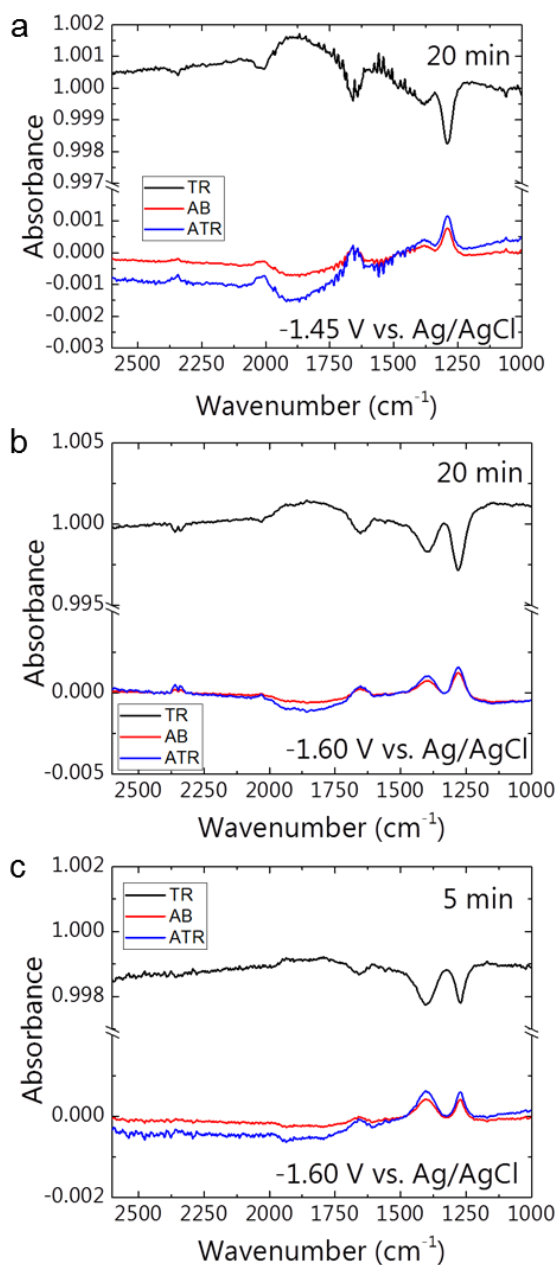
Figure A8. ATR-FTIR spectra shown in transmission (TR), absorbance (AB) and attenuated total reflectance (ATR). (a) spectra measured at -1.45 \text{ V} at saturated \text{CO}_2 , (b) spectra measured at -1.60 \text{ V} at saturated \text{CO}_2 and (c) spectra measured at -1.60 \text{ V} at low \text{CO}_2 concentration.
