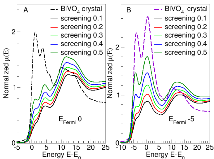
Figure D7. Simulated O K edge spectra. The effect of changing the screening parameter on the \text{BiVO}_4 crystal structure for (a) a standard and (b) a 5 eV shifted Fermi level case.
