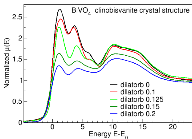
Figure D6. The effect of increasing the dilatorb parameter on the \text{BiVO}_4 crystal structure.
