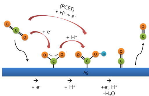
Figure 2.9. Schematic depiction of proposed reaction mechanism of \text{CO}_2 reduction to CO on a thin film Ag catalyst. At most applied potentials, the 1 step PCET mechanism leads to the formation of CO on the Ag thin film catalyst. At -1.6 V the 2-step reaction mechanism is dominant.
