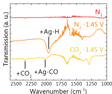
Figure 2.5. Assignments of reactants and products present during ATR-FTIR experiments in 0.1 M KCl. A full experimental procedure is shown: the red line is a spectrum taken during \text{N}_2 flow where the background was also taken during \text{N}_2 to make sure the system is in equilibrium. The orange spectrum is taken 20 min after a potential of -1.45 V is applied with the red line as background spectrum. The red spectrum is taken 20 min after \text{CO}_2 is introduced to the cell with 30 min \text{N}_2 at -1.45 V as background spectrum.
