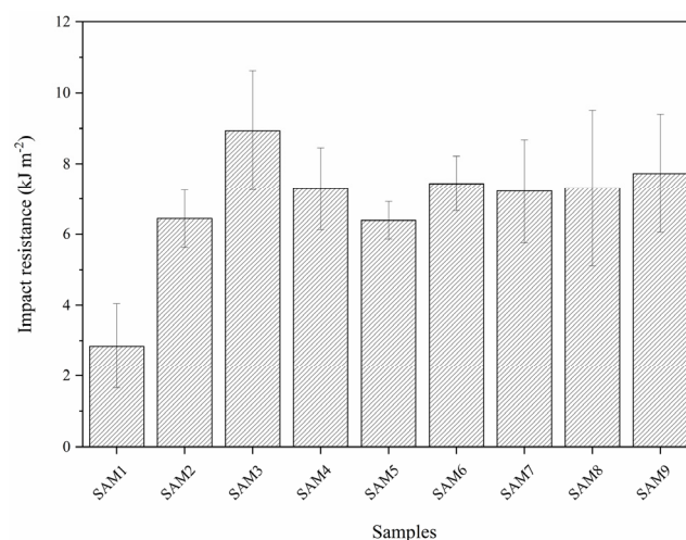
Figure 9. Impact resistance analysis of composites and neat matrix.
