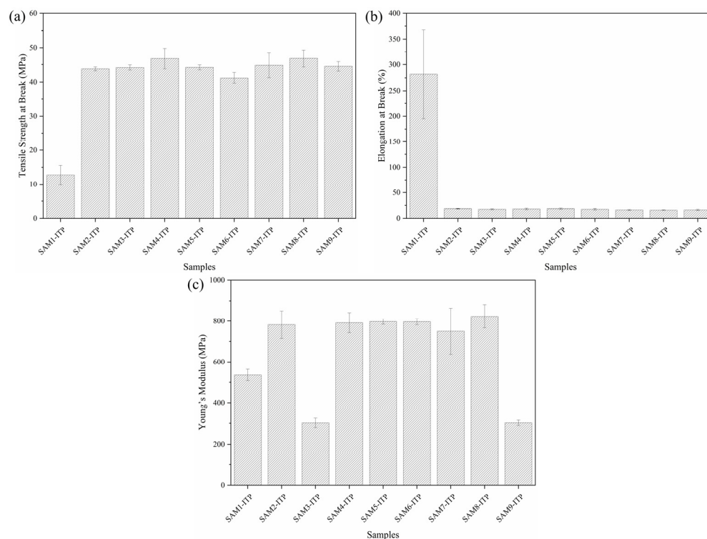
Figure 7. Tensile strength at break (a), elongation at break (b), and Young's modulus (c) of composites samples manufactured via the thin-plate injection process.
