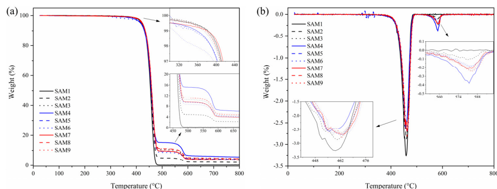
Figure 4. (a) TGA and (b) DTG analyses of the composites compared to the neat PP matrix.
