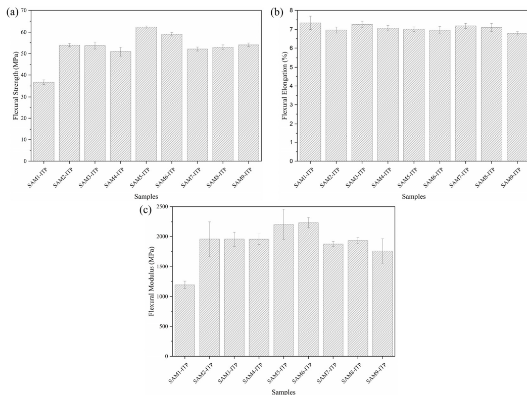
Figure 8. Flexural resistance (a), flexural elongation (b), and flexural modulus (c) for composite samples produced via the thin-plate injection process.
