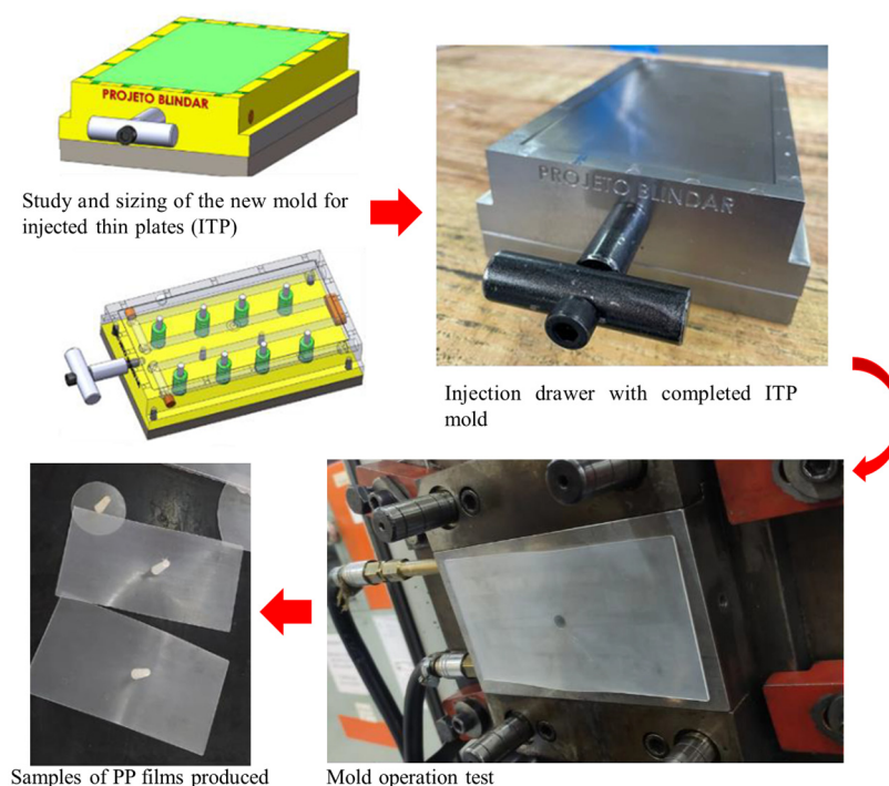
Figure 2. Development of the mold for thin-plate injection.
