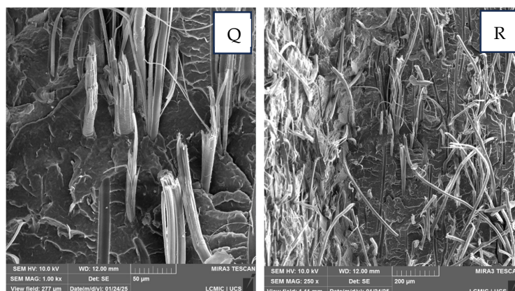
Figure 6. Scanning electron microscopy (SEM) of composites and neat matrix at two different magnifications indicated in the images: 50 \mu\text{m} and 200 \mu\text{m} . (A,B) AM1, (C,D) AM2, (E,F) AM3, (G,H) AM4, (I,J) AM5, (K,L) AM6, (M,N) AM7, (O,P) AM8, and (Q,R) AM9.
