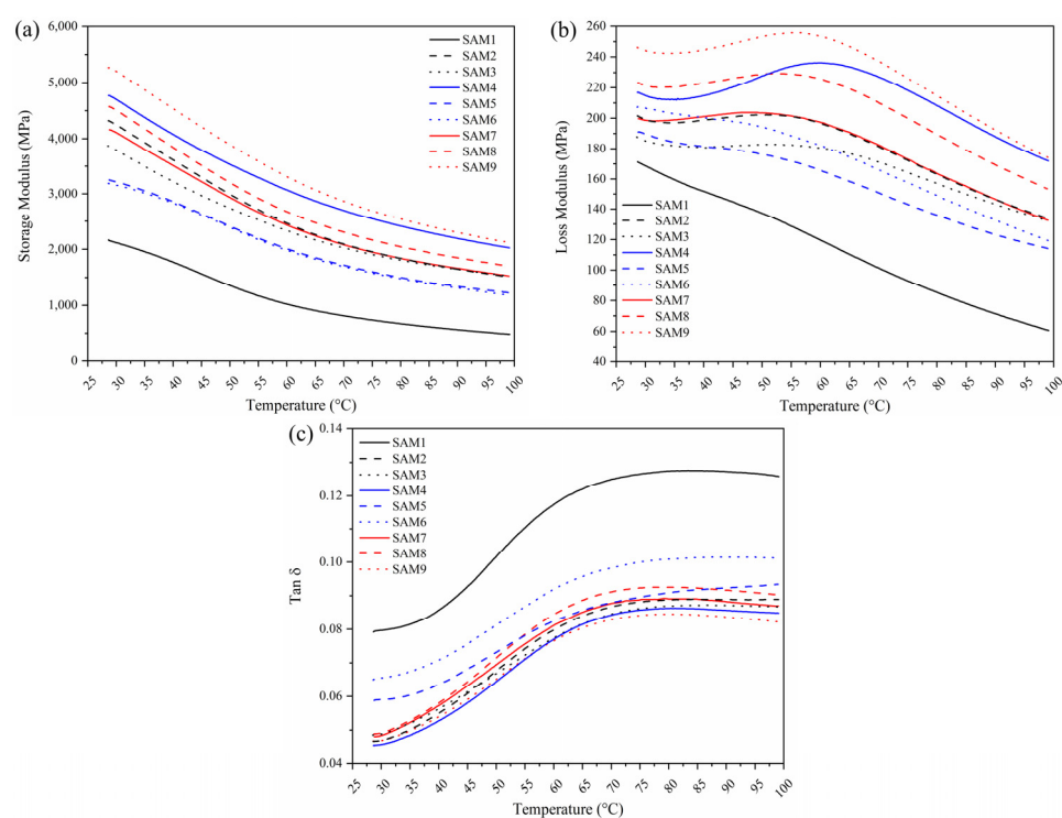
Figure 3. Storage modulus (a), loss modulus (b), and tan \delta (c) of neat polypropylene and composite samples containing aramid fibers, graphene nanoplates (GNPs), and MAPP.
