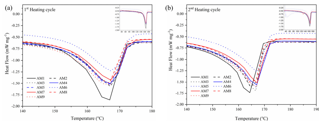
Figure 5. DSC analysis of (a) first heating cycle and (b) second heating cycle for the neat PP matrix and composite samples.
