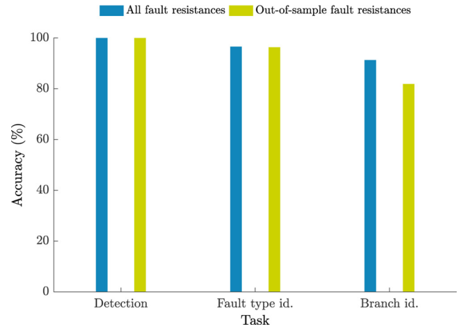
Fig. 10. Comparison of the average accuracy of the three tasks between all studied fault resistances between 3 and 500 \Omega and the out-of-sample fault resistances.
