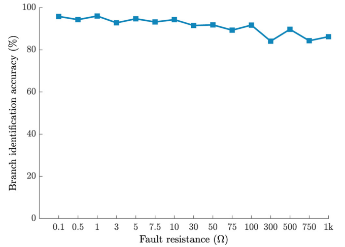
Fig. 8. Faulty branch identification accuracy in the test dataset for different fault resistance values.
