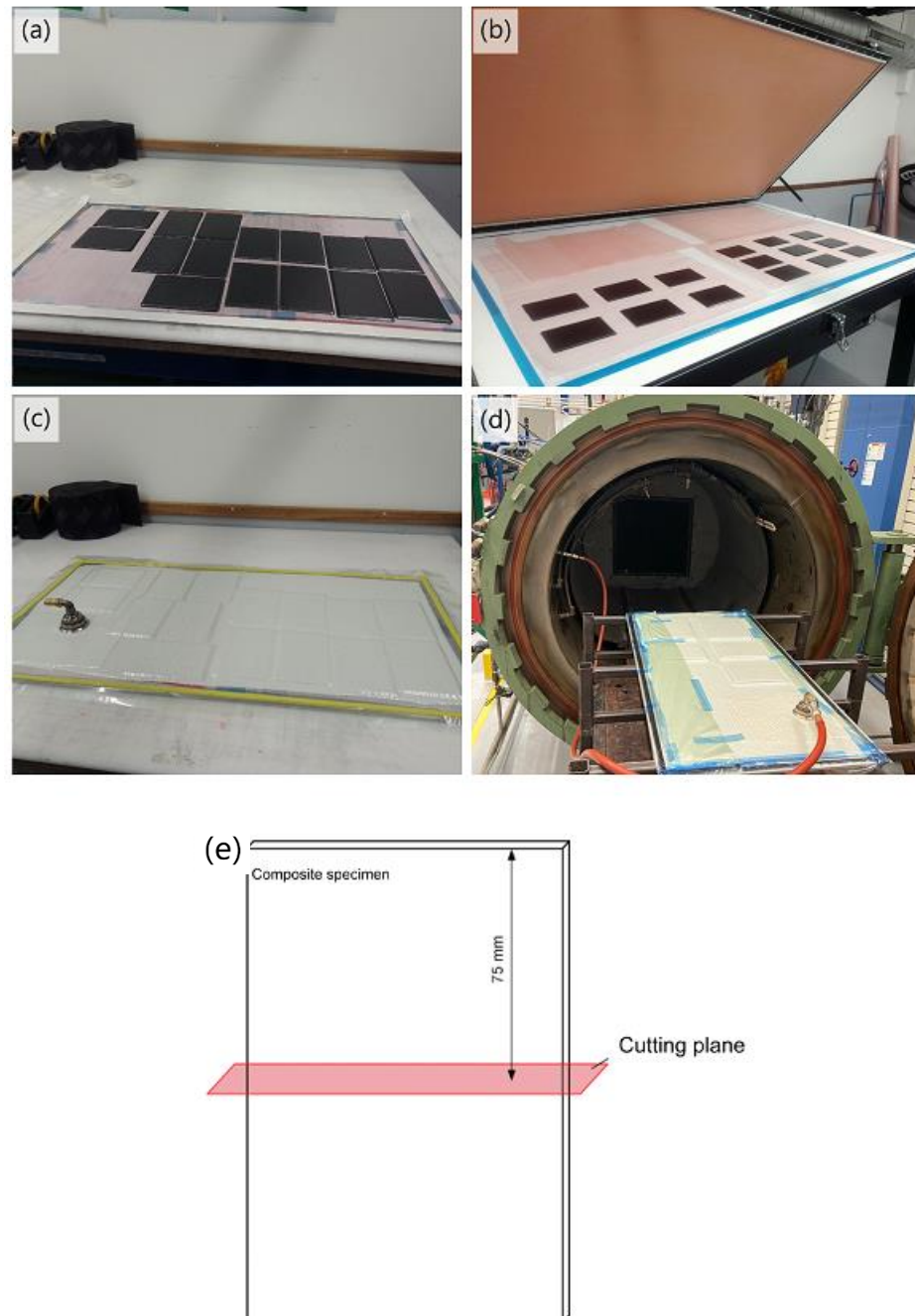
Figure 3. Manufacturing process: (a) cutting the preregs into standard specimen size and stacking the layers, (b) applying pressure after stacking every four layers to ensure there is no air or bubbles, (c) completing the vacuum-bag lay-up, (d) curing at autoclave under desired temperature and pressure, (e) cutting plane for examining the cross-section of the impacted specimen.
