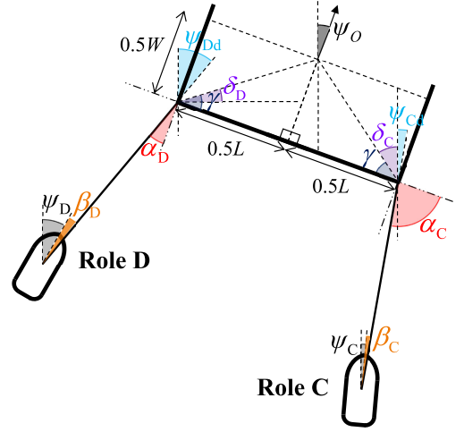
Fig. 7. Desired geometrical configuration for the rear tugs.
