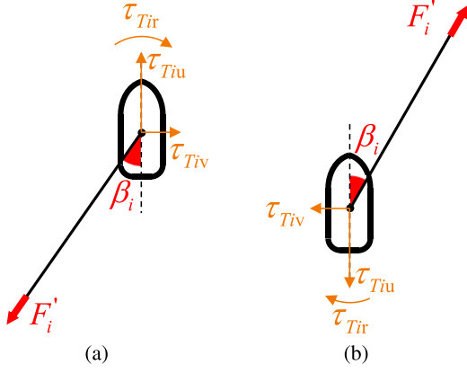
Fig. 3. Force diagram of the tugs. (a) Role A and B. (b) Role C and D.
