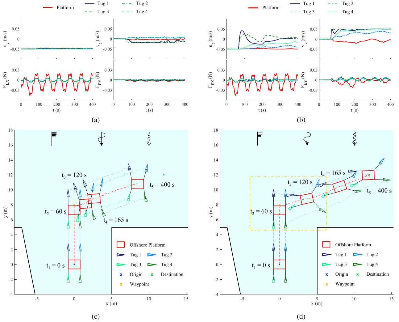
Fig. 8. Towing processes under environmental disturbances in two scenarios. (a) Current velocities ( u_c , v_c ) and wind and wave-resultant forces ( F_{EX} , F_{EY} ) on x- and y-axis in the body-fixed frame of Scenario I. (b) Current velocities ( u_c , v_c ) and wind and wave-resultant forces ( F_{EX} , F_{EY} ) on x- and y-axis in the body-fixed frame of Scenario II. (c) Towing process in Scenario I. (d) Towing process in Scenario II.
