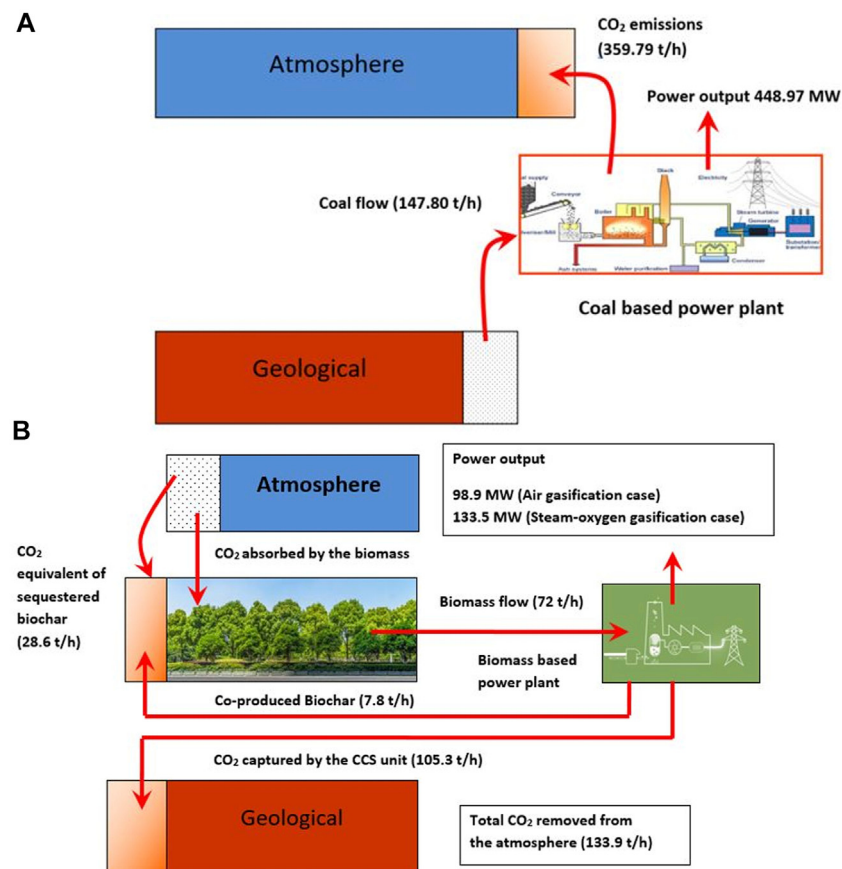
FIGURE 8 | (A) Main CO 2 flows in a typical coal-based power plant. (B) Main CO 2 flows in the BECCS including biochar addition to soil for the 10% biochar co-production in the given biomass feed.
