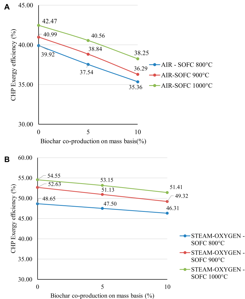
FIGURE 7 | (A) Effect of different operating temperatures of the SOFC on CHP exergy efficiency for the air gasification case. (B) Effect of different operating temperatures of the SOFC on CHP exergy efficiency for the steam-oxygen gasification case.
