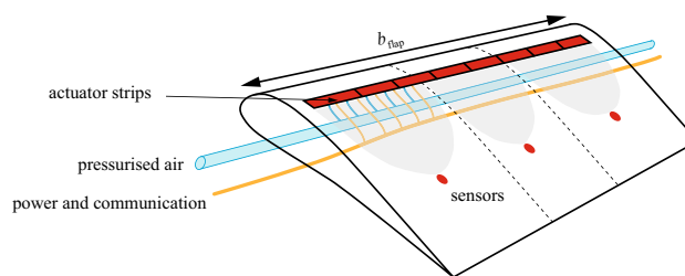
Fig. 2 Schematic representation of PJA implementation in a flap
